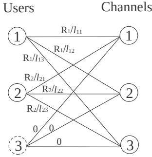
Fig. 1: An illustration of reduction of MPCA with linear rate function to minimum-weight bipartite matching for M = 2 (with user three as a dummy user) and N = 3 .
