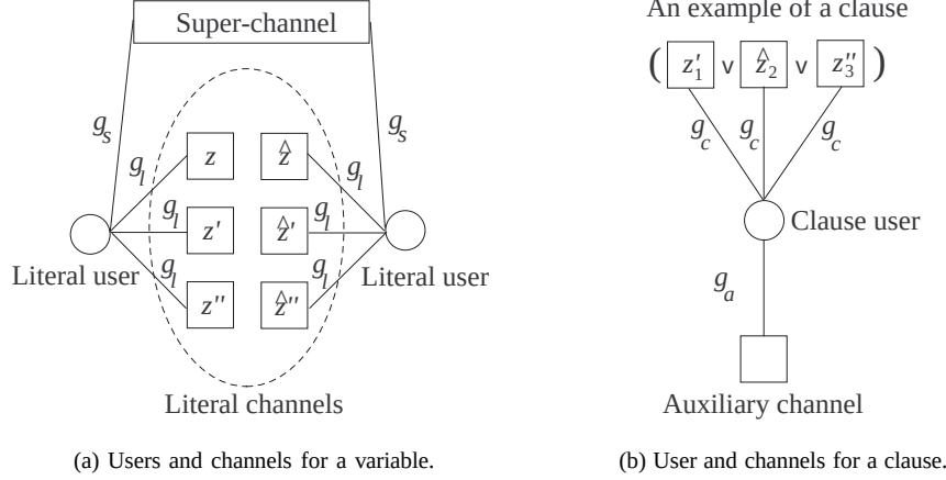
Fig. 2: An illustration of problem reduction.
