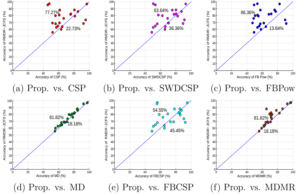
Fig. 5. Pair-wise scatter plot of the accuracies of our proposed method (Prop.) versus other classification methods. In the figure, each dot represented the classification accuracy of a subject. The results demonstrated that our proposed method achieved higher accuracies compared with other methods, i.e., most points lied above the diagonal line.
