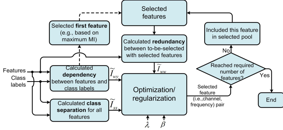
Fig. 6. Schematic illustration of the proposed feature selection process.
