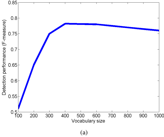
Fig. 5 The relationship between the scene text detection performance and the vocabulary size of the learned code-book.
