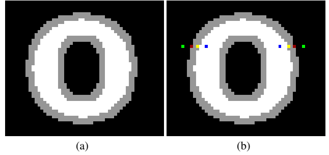
Fig. 4 Illustration of scene text segmentation based on the text boundary: (a) the internal and external text boundaries for character O; (b) candidate text and background pixels detected.
