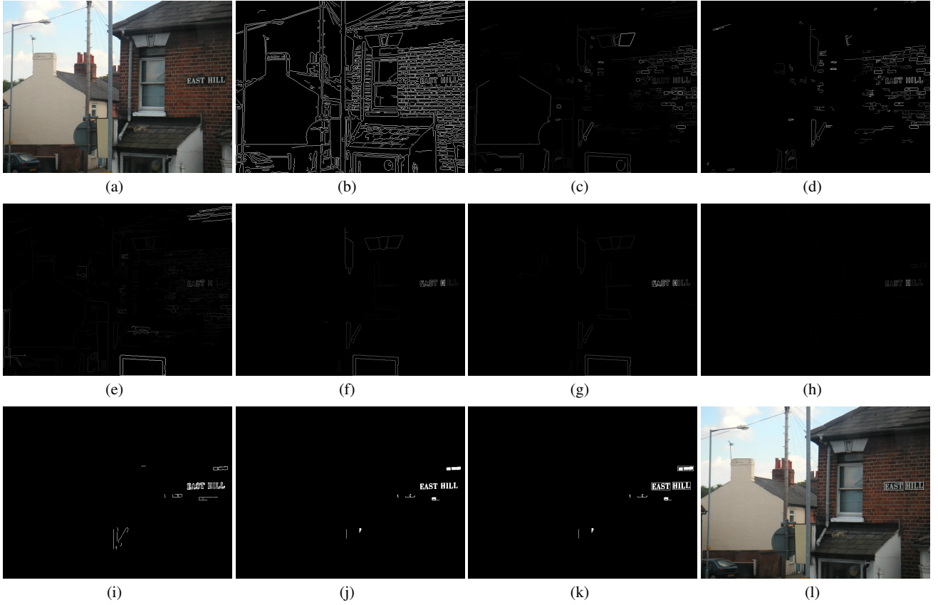
Fig. 2 The process of the proposed scene text localization technique: For the sample image in Fig. 2(a), Figs. 2(b)-2(e) show the detected Canny edges and the three text-specific features, respectively. Figs. 2(f)-2(h) show the combined features (channel Y at the original image scale) and the integration across multiple image channels and multiple image scales, respectively. Figs. 2(i)-2(k) show the extracted text boundary, the segmented text, and the detected word candidates, respectively. Fig. 2(l) shows the finally located words within the original scene image (after the false alarm removal using the supported vector regression (SVR) to be described in Section 2.4.)
