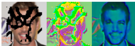
Fig. 4: From left to right, we show the input masked image, masked semantic feature after CLIP encoder, and semantic feature after SIR.
