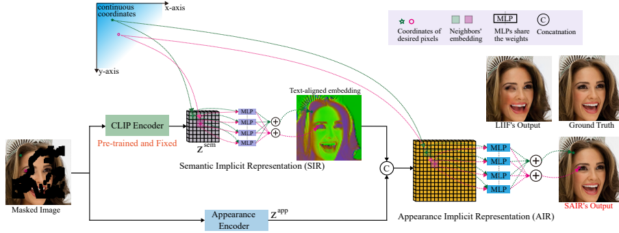
Fig. 2: Pipeline of our semantic-aware implicit representation (SAIR). The semantic implicit representation (SIR) is used to complete the missing semantic information. The appearance implicit representation (AIR) is used to complete missing details
