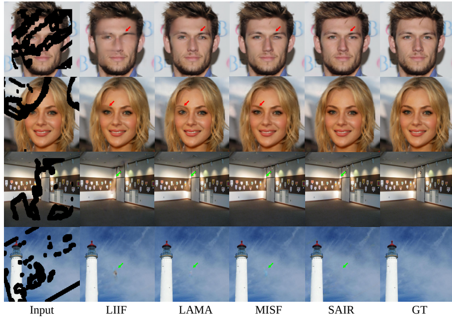
Fig. 3: Visual comparison with competitors: the first two cases are from the CelebAHQ dataset, while the last two are from the ADE20K dataset.
