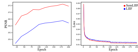
Fig. 5: PSNR vs Epoch and Training Loss vs Epoch.
