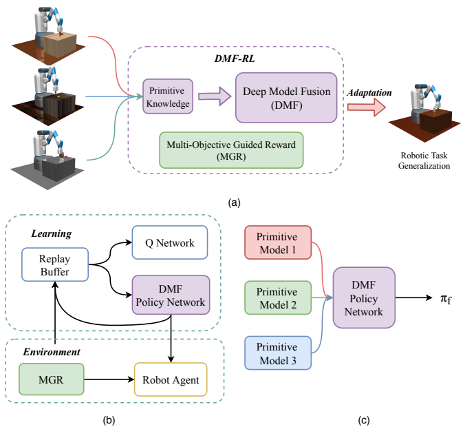
Fig. 1: (a) The DMF-RL system that combines the knowledge from previous learned model for efficient robotic task generalization (b) The robot agent learning structure using DMF-RL system (c) DMF policy network structure
