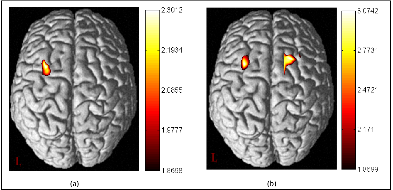
Figure 2. Activation maps of HbO with averaged trials. Each map depicts the significant difference between (a) motor imagery and idle state. (b) passive movement and idle state with threshold p < 0.05 . Significant activation can be observed either ipsilaterally (a) or bilaterally (b) in the sensorimotor area.
