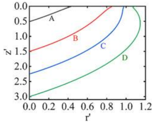
Fig. 4. Contours of \tau_{max} in the material calculated from the Hertzian contact relations for a sphere in elastic contact with a flat surface.
