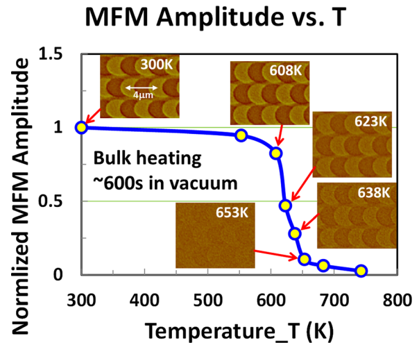
FIG. 4. Plot of MFM amplitude vs. bulk heating temperature. Insets: MFM images for thermally degraded/erased magnetic patterns for T = 300, 608, 623, 638, 653\text{ K} . Note that the crescent shape of the pre-recorded “+” and “-” \mu\text{m} sized magnetic patterns is due to the sequential overlap of the circularly shaped dot patterns over previously recorded dot patterns.
