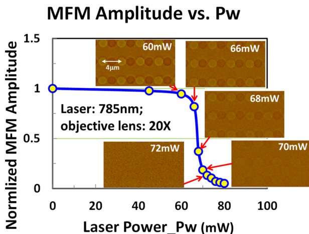
FIG. 3. Plot of MFM amplitude vs. scanning laser power. Insets: MFM images for thermally degraded/erased magnetic patterns for P_w = 60, 66, 68, 70, 72\text{ mW} .
