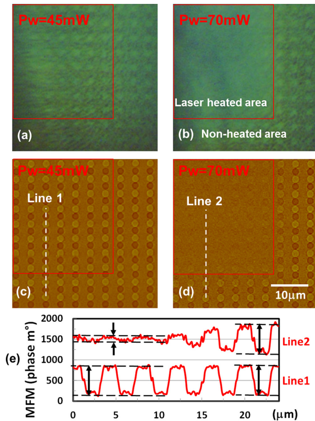
FIG. 2. Kerr magnetic images (a) and (b) and MFM images (c) and (d) for thermal erasure of pre-recorded magnetic patterns by scanning laser beam with P_w = 45\text{ mW} and 70\text{ mW} . (e) MFM line profiles of line 1 and line 2 in (c) and (d).
