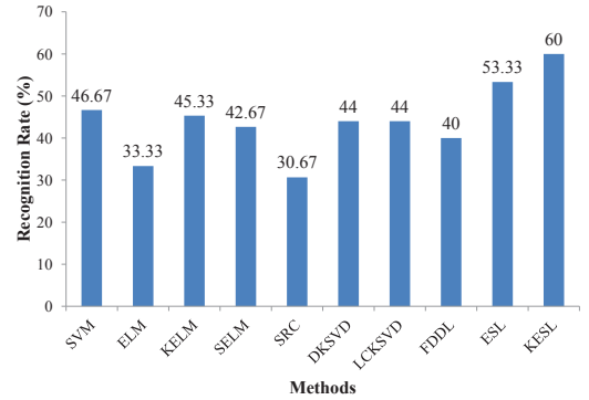
Fig. 8. Comparison of accuracy when the different classifiers are trained on the original CK+ database and applied to data collected by us, which includes occlusion, head posed variations, and illumination changes.
