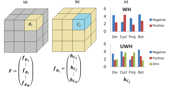
Fig. 3. Spatio-temporal descriptor construction. (a) Volume data is divided into a number of 3D blocks ( \mathbf{B}_m ) and the final descriptor ( \mathbf{y} ) is a concatenation of features from all the blocks. (b) Each block is further divided into number of 3D cells ( \mathbf{C}_n ) and the feature vector of each block ( \mathbf{f}_{\mathbf{B}_m} ) is a concatenation of all the cell histograms within that block. (c) Weighted and un-weighted histograms are calculated for each cell based on the four spatio-temporal features and concatenated to obtain the cell histogram.
