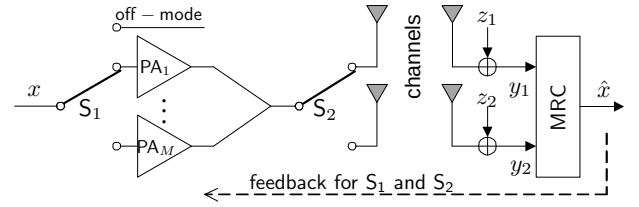
Fig. 3. A TAS-MRC system model with the proposed PA switching (PAS), in which switch S_1 selects a PA and switch S_2 selects a transmit antenna.
