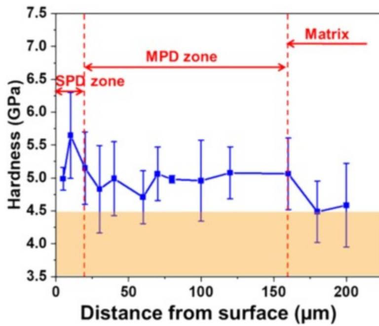
Fig. 15. Variations of hardness as a function of distance from the surface of the 200 \mu\text{J} sample.
