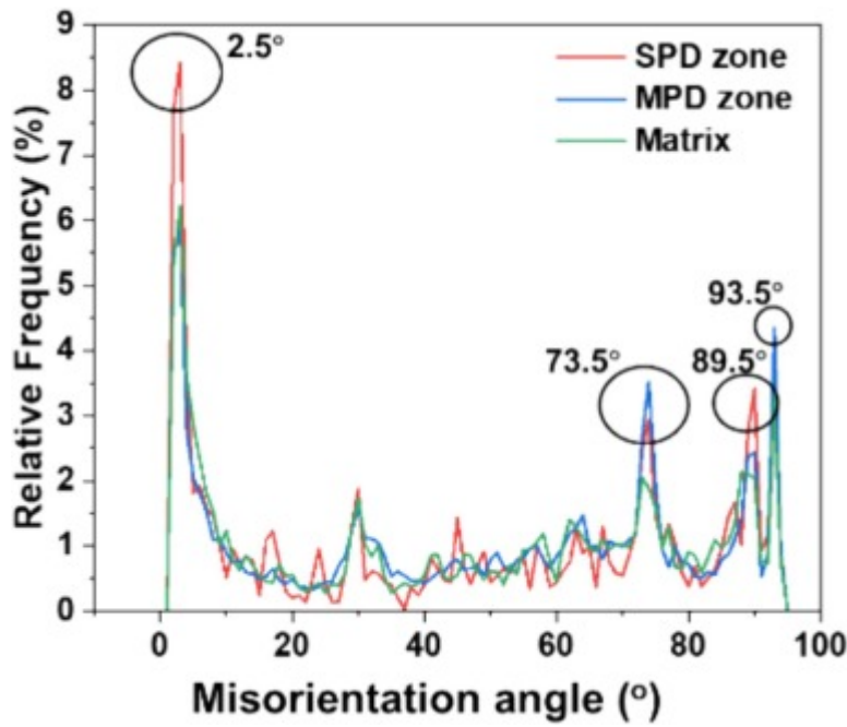
Fig. 17. Grain boundary misorientation angle distribution of a phase at different zones in the 200 \mu J sample.
