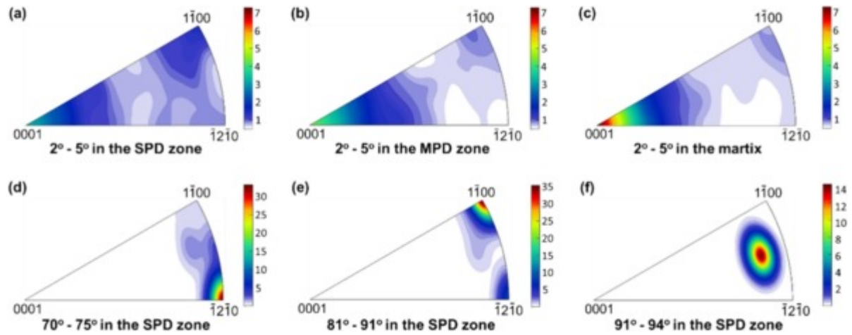
Fig. 17. Grain boundary misorientation angle distribution of a phase at different zones in the 200 \mu J sample.
