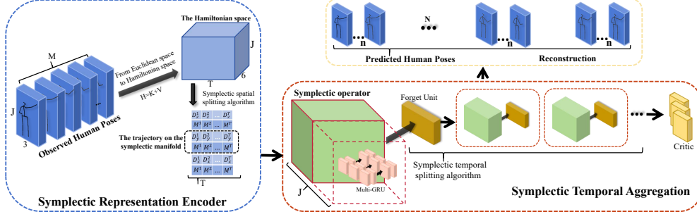
Figure 2. The proposed Symplectic Integral Neural Network (SINN) architecture.
