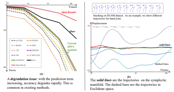
Figure 1. Illustration of human motion prediction challenges. (a) Existing methods suffer from significant long-term performance degradation. (b) Conventional motion representation is not numerically stable.
