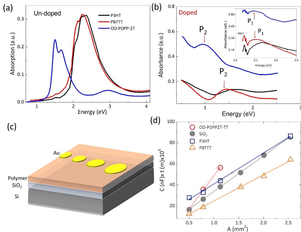
Fig. 2: UV-Vis spectra and dielectric measurement of P3HT, PBTTT-C 14 and OD-PDPP2T-TT polymers (a) UV-Vis spectra of the pristine and (b) Doped P3HT, PBTTT-C 14 and OD-PDPP2T-TT polymer thin films with 0.03M concentration of FeCl 3 . Inset of figure (b) shows FTIR spectra of doped samples. (c) Schematic of the measurement geometry and the dielectric constant of different conjugated polymer films. (d) Capacitance (C) × thickness (t) of polymer thin films as a function of area (A) for un-doped P3HT (blue squares), PBTTT (orange triangles) and OD-PDPP2T-TT (red circles) and SiO 2 (grey circles). Thin films of P3HT, PBTTT-C 12 and OD-PDPP2T-TT polymer were prepared by spin coating in di-chlorobenzene solution.
