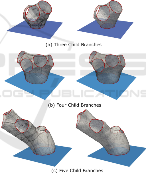
Figure 9: Tree Joint Meshes. The following tree joint meshes were created randomly with varying number of child branches. The original mesh created using CGAL's skin surface is shown on the left, while the resmoothed version is shown on the right.
