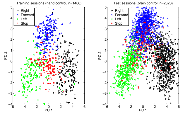
Fig. 3. Same way of visualization as in Fig. 1. Analysis was performed on data set C20140219
