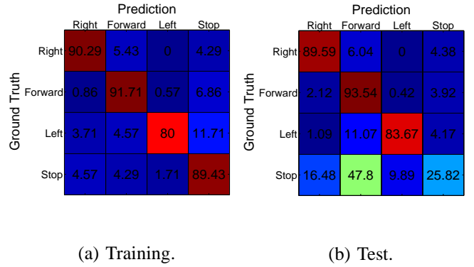
Fig. 4. Comparison of the confusion matrices of both training and test sessions from data set C20140219.
