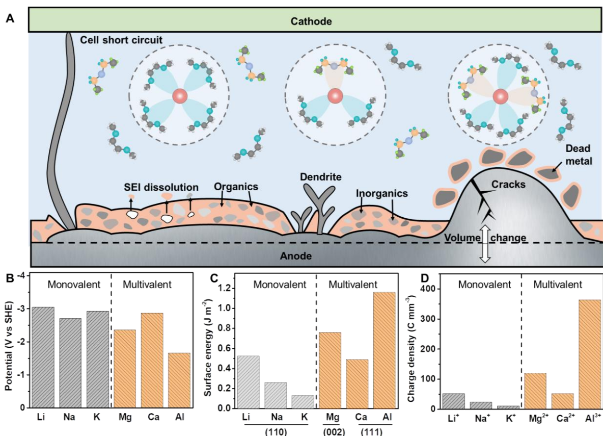
Fig. 1. Common challenges for monovalent and multivalent metal anodes. (A) Schematic showing the challenges for monovalent and multivalent metal anodes in conventional nonaqueous electrolytes, including uncontrolled growth of dendrite, spontaneous decomposition of electrolyte solvation structure, and subsequent formation of structurally inhomogeneous and compositionally unoptimized solid electrolyte interphase (SEI). During repeated plating and stripping, the organic and inorganic SEI components will dissolve in the electrolytes, and the huge volume change will cause SEI cracking and trigger the formation of electrochemically isolated “dead” metal. Meanwhile, the growth of metallic dendrites can proliferate in the interelectrode space to bridge the electrodes, giving rise to an early short-circuit cell failure in a working battery. These challenges are highly related to the intrinsic properties of monovalent and multivalent metal anodes and their coupled charge carriers, including (B) redox potential, (C) surface energy, and (D) charge density. Data obtained from (1, 151).
