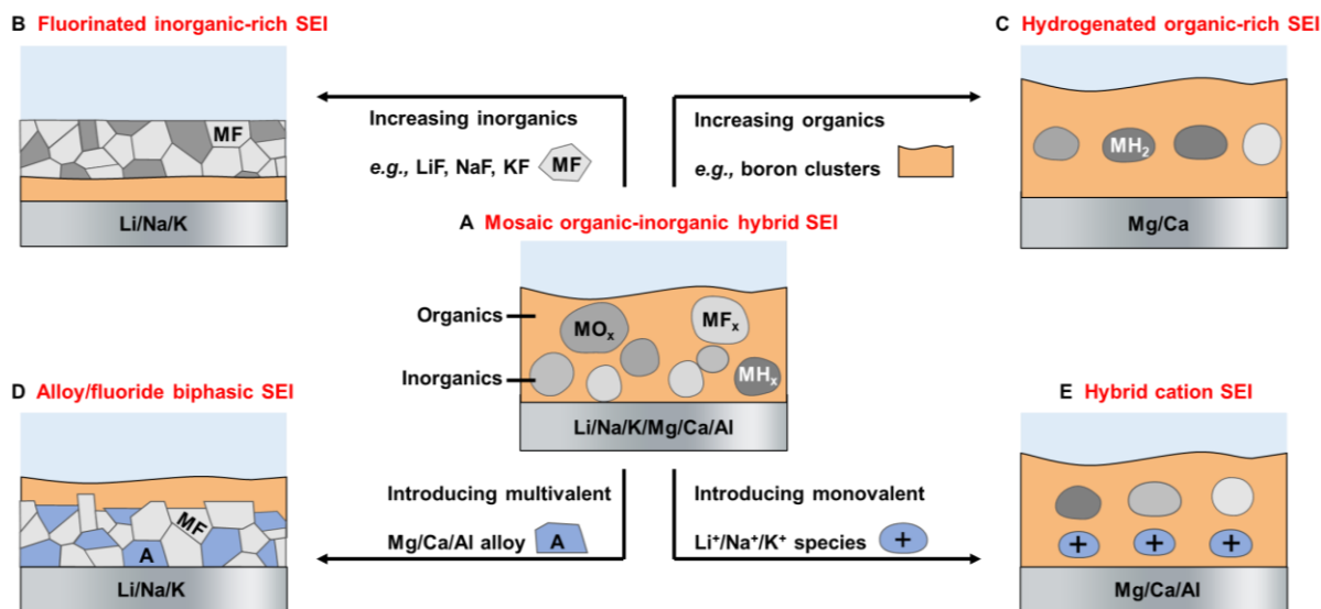
Fig. 4. Solid electrolyte interphase for monovalent and multivalent metals. Schematic showing (A) similar mosaic organic-inorganic hybrid SEI layers on Li, Na, K, Mg, Ca, and Al metal anodes. These structurally heterogeneous SEI layers trigger anisotropic ion transfer and uneven stress distribution, thereby leading to uncontrolled dendritic formation and early electrode failures. Schematic showing optimal (B) fluorinated inorganic-rich and (D) alloy/fluoride biphasic bilayer SEI layers for Li, Na, and K metal anodes, (C) hydrogenated organic-rich and (E) hybrid cation SEI layers for Mg, Ca, and Al metal anodes. These optimized SEI layers possess some universal merits of high ion conductivity, electronic insulation, (electro)chemical stability, and mechanically rigid-flexible synergy.
