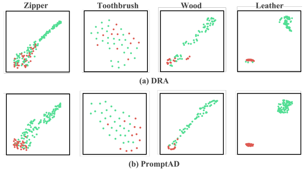
Figure 4. Visualizations of features learned by DRA and our proposed PromptAD on the unseen test classes of MVTec dataset. Green indicates anomalies while red indicates normal samples. Features learned by PromptAD show better separability.
