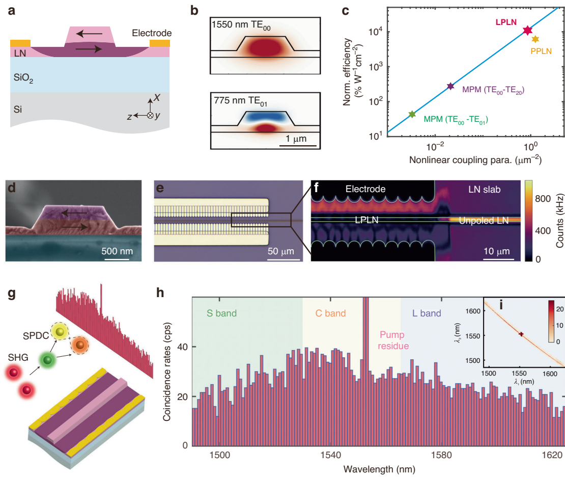
Fig. 1 Layer-poled lithium niobate (LPLN) nanophotonic waveguide for efficient photon-pair generation. a Schematic of LPLN waveguide cross-section in x-cut TFLN. Dark and light pinks indicate inverse domain polarities. b Mode profiles ( E_z component) of TE_{00} mode at 1550 nm and TE_{01} mode at 775 nm for MPM. c Theoretical comparison of normalized SHG conversion efficiency among different nonlinear TFLN waveguide schemes, including LPLN (red), PPLN (yellow), MPM between TE_{00} at FH and TE_{20} at SH (purple), and MPM between TE_{00} at FH and TE_{01} at SH without poling (green). The blue line is normalized SHG efficiency versus nonlinear coupling parameter, a measure of mode overlap considering \chi^{(2)} polarity distribution, with MPM condition. d A false-colored scanning electron micrograph of a LPLN waveguide cross-section, showing the electrical poling induced inverse polarities. e A top-view optical micrograph of a fabricated LPLN waveguide. f Top-view laser-scanning SHG imaging of a LPLN waveguide, where the unpoled waveguide is bright but the poled waveguide becomes dark due to the destructive interference of SH signals from the inversely polarized LN layers. g Schematic of cascaded SHG-SPDC processes for photon-pair generation. h Coincidence spectrum measured from 1486 nm to 1625 nm, covering telecom S, C, and L bands. i Joint spectral intensity of the photon pairs. The dark cross is due to the residual pump noise
