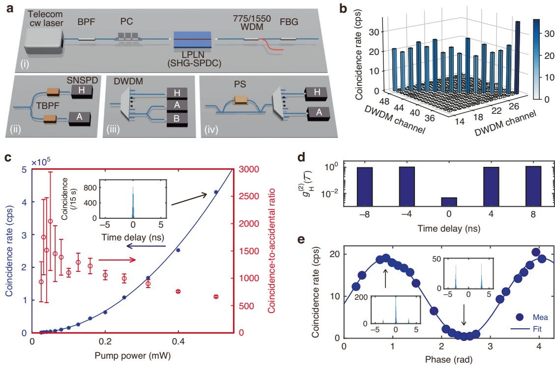
Fig. 3 Non-classical characterization of photon-pair generation in a LPLN nanophotonic waveguide using a cascaded SHG-SPDC scheme. a Experimental setup for (i) photon-pair preparation, (ii) broadband photon spectral characterization, (iii) pair-generation rate, CAR, and heralded correlation measurements, and (iv) two-photon interference measurement. BPF: bandpass filter; PC: polarization controller; WDM: wavelength division multiplexer; FBG: fiber Bragg grating; TBPf: tunable BPF; SNSPD: superconducting nanowire single-photon detector; DWDM: dense wavelength division multiplexer; PS: phase shifter. b Joint spectral intensity constructed by correlation measurement over 32 DWDM channels (ITU frequency Ch14-Ch29 and Ch48-Ch53), revealing strong frequency correlation through coincidences exclusively along the diagonal elements in the 16 \times 16 matrix. c Measured (blue dots) and quadratically fitted (blue line) on-chip photon-pair generation rate and coincidence-to-accidental ratio (red) as a function of on-chip pump power. A raw coincidence histogram measured for 15 seconds is shown in the inset. d Heralded second-order correlation function measured at various time delays at a pump power of 0.5 mW. The correlation is 0.008 \pm 0.002 at zero time delay, indicating the measurements are in the single-photon regime. e Two-photon interference measured at a pump power of 0.5 mW, and the measured visibility yields 98.0%. Raw coincidence histograms at constructive and destructive interference are shown in the insets. Measurements in c-e are all done between Ch21 and Ch41
