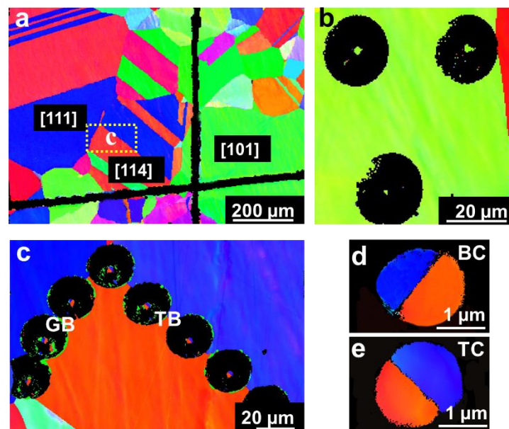
Figure 1. Representative EBSD micrographs. (a) Area from where the micropillars were fabricated. The black unindexed lines are scratch marks utilized to locate the area
