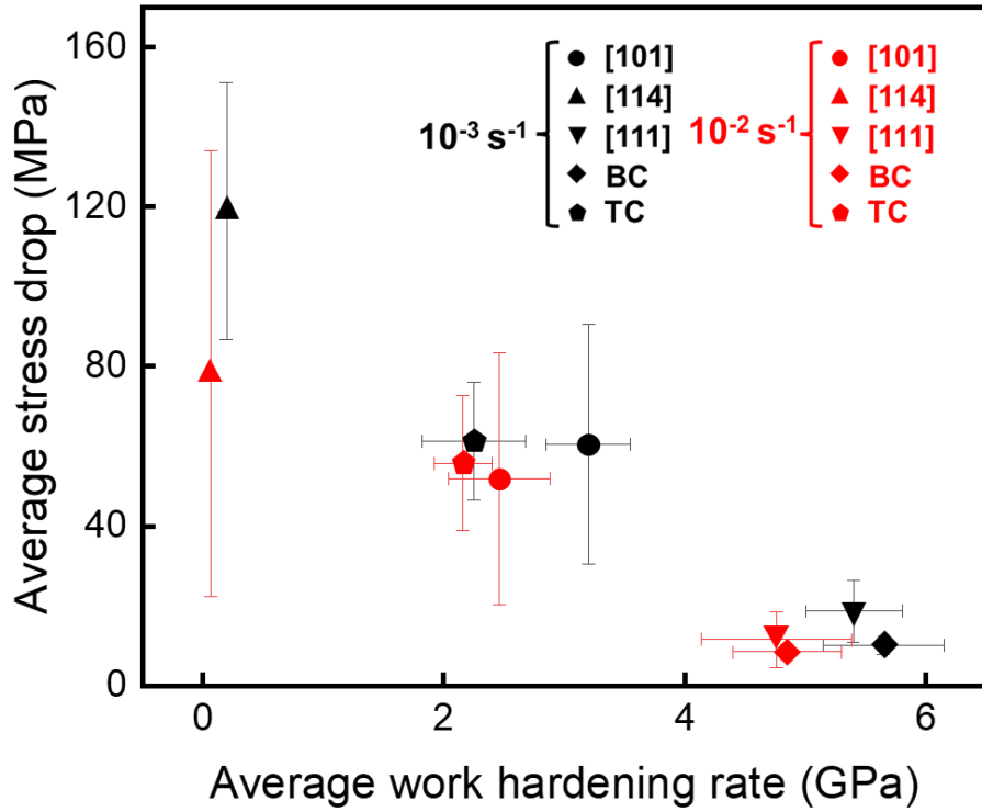
Figure 10. Variation of the average stress drop magnitude with the average work hardening rate at the strain rates of 10^{-2} and 10^{-3} s^{-1} for different micropillars tested in this work: [111], [114], [101] SC pillars and [111]/[114] BC and TC pillars.
