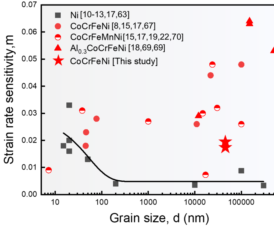
Figure 13. Variations of the strain-rate sensitivity ( m ) and grain size ( d ). Literature data for pure Ni [10-13,17,63], along with CoCrFeNi [8,15,17,67], CoCrFeMnNi [15,17,19,22,70], and Al 0.3 CoCrFeNi HEAs [18,68,69].
