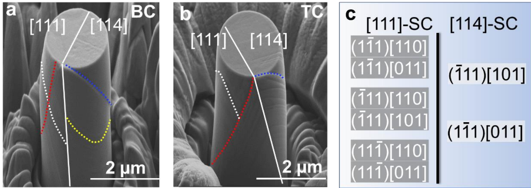
Figure 7. Morphologies of the compressed (at \dot{\epsilon} = 10^{-3} \text{ s}^{-1} ) (a) BC and (b) TC micropillars, with (c) the corresponding list of the activated slip systems in both the pillars.
