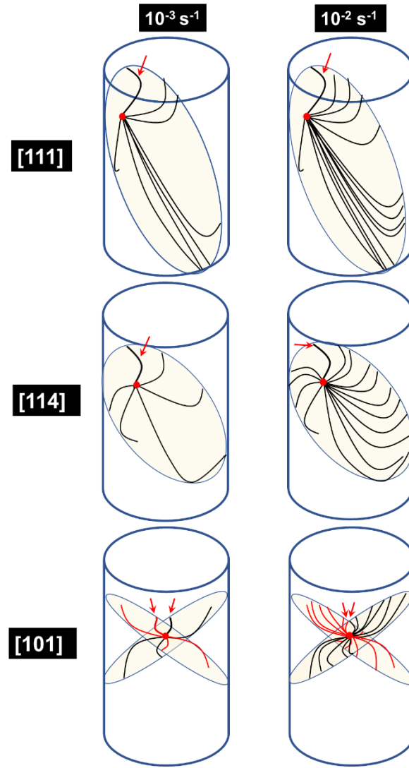
Figure 12. Schematic illustrations of the dislocation density evolution at 10^{-3} and 10^{-2} \text{s}^{-1} strain rates in the [111], [114], and [101] SC pillars. Red dots represent the dislocation pinning points and red arrows point out the single-arm dislocation source.
