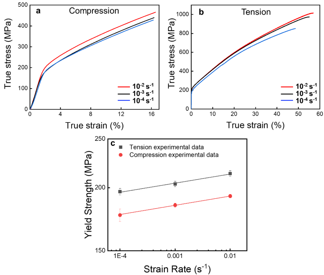
Figure 4. Representative true stress–true strain responses obtained from the uniaxial (a) compression and (b) tension tests on the PC specimens. (c) Double logarithmic plots of the yield strength versus strain rate for both compression and tension tests. The lines mark the linear fits of the double logarithmic plots.
