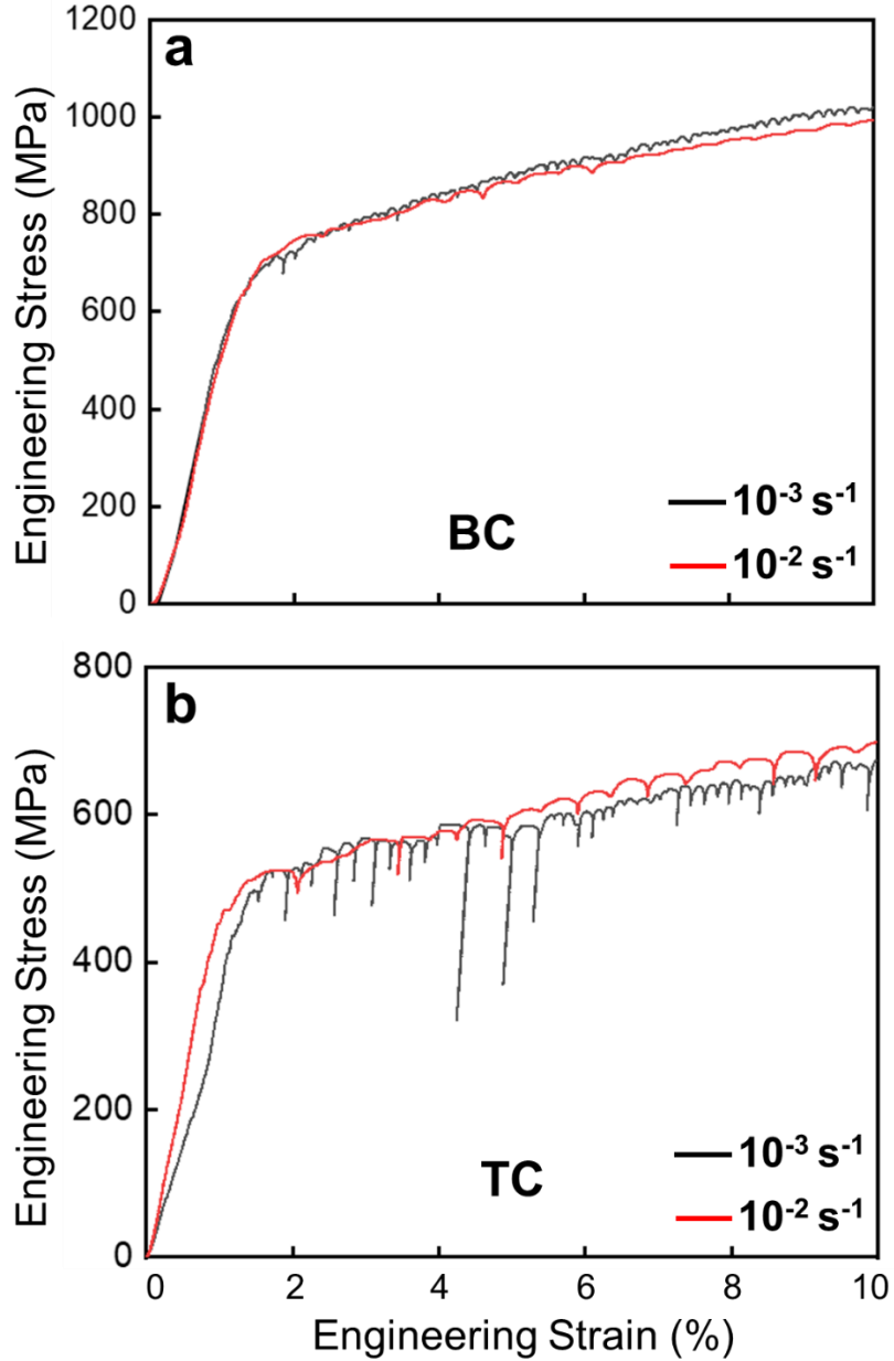
Figure 8. Representative engineering stress–strain responses of (a) BC and (b) TC micropillars subjected to uniaxial compression at 10^{-2} and 10^{-3} \text{ s}^{-1} strain rates.
