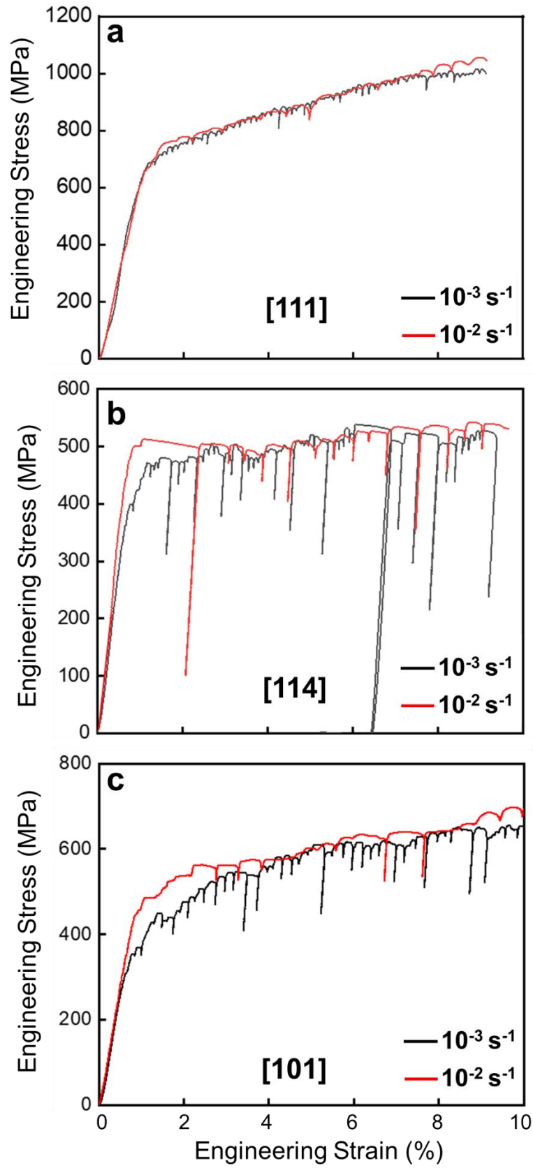
Figure 6. Representative engineering stress-strain responses of (a) [111], (b) [114], and (c) [101] SC micropillars subjected to uniaxial compression at 10^{-2} and 10^{-3} \text{ s}^{-1} strain
