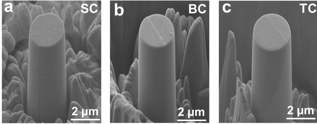
Figure 2. Representative SEM images of the as-fabricated (a) [111]-oriented SC , (b) BC , and (c) TC pillars, respectively.
