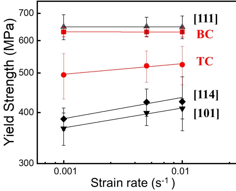
Figure 9. Double logarithmic plots of yield strength versus logarithmic strain rate for different micropillars tested in this work: [111], [114], [101] SC pillars and [111] / [114] BC and TC pillars.
