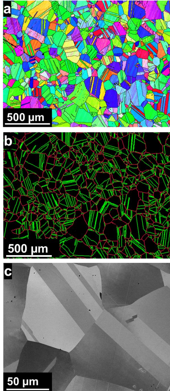
Figure 3. Representative microstructures of the CoCrFeNi HEA showing (a) an EBSD IPF map, (b) the boundary distribution (where red and green lines represent the high-angle grain boundaries and the twin boundaries, respectively), and (c) a higher magnification BSE image of the microstructure.
