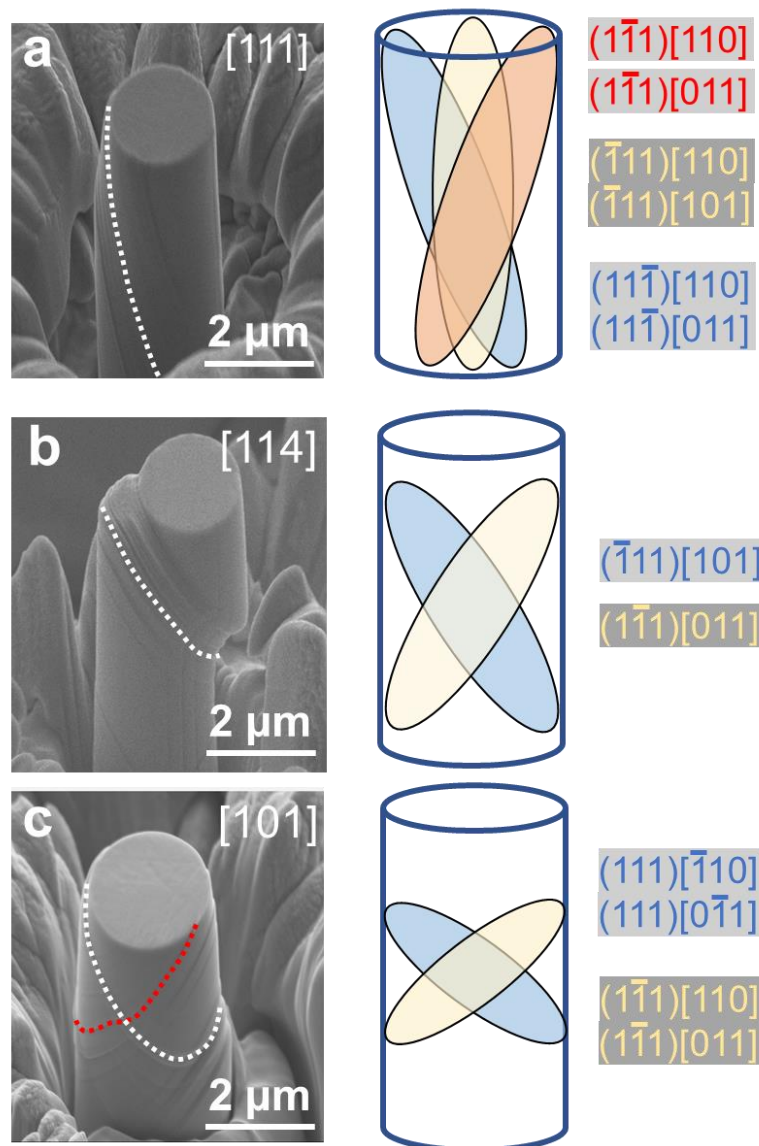
Figure 5. Morphologies of the compressed SC pillars, characterized by SEM and schematics of the slip systems with the maximum Schmid factors, SF_{max} . (a) [111], (b)
