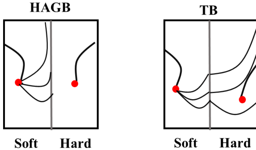
Figure 11. Schematic illustrations of the effects of high-angle grain boundary (HAGB) and twin boundary (TB) on the dislocation motion.
