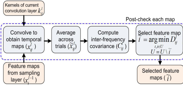
Fig. 3. Illustration of the frequency complementary map selection (FCMS) scheme.
