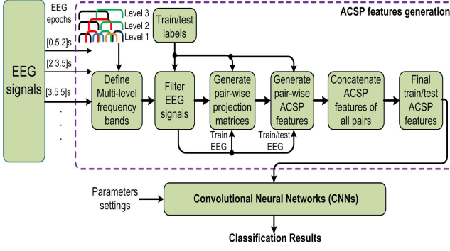
Fig. 1. Schematic illustration of the proposed CMI-ACSP-CNN s scheme.
