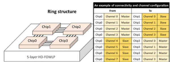
Fig 2. Integration of four chiplets, and an example of channel connection and configuration.
