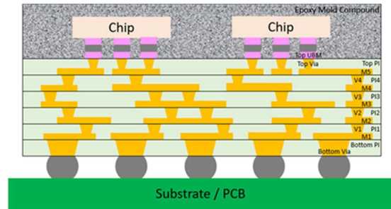
Fig. 3. Illustration of the five layer RDL FOLWP package
