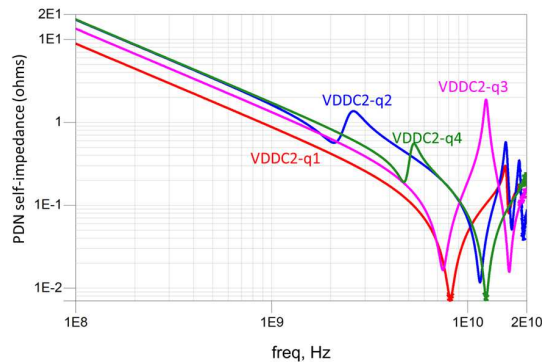
Fig. 13. Simulated PDN self-impedance for the VDDC2 in the four quadrants of the package.
