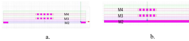
Fig. 8. High density bus cross section structure: a. the return path is constrained; b. the return path is a full metal plane.
