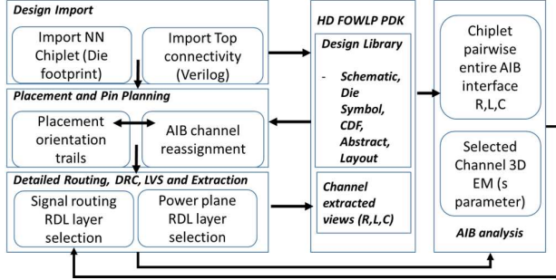
Fig. 7. Interconnect aware SIP reference design flow.
