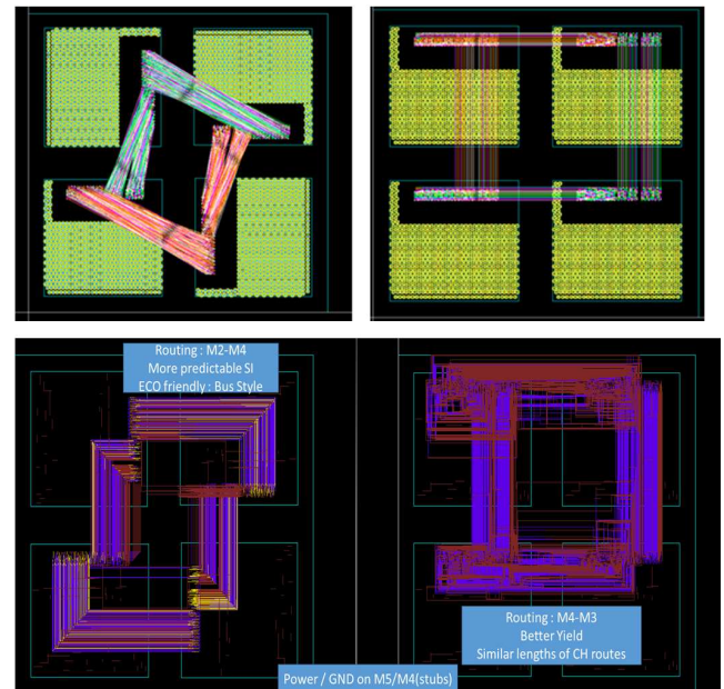
Fig. 6. Four NN accelerator chiplet configurations with different chiplet placement trials
