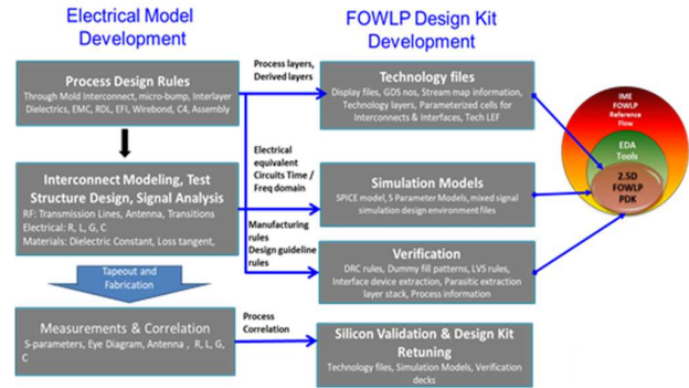
Fig. 5. HD FOWLP PDK development process, supporting upstream design tools from Cadence, verification checks using Mentor (Siemens) tools and system analysis tools from Keysight
