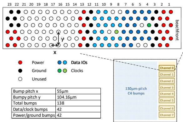
Fig. 4. AIB channel bump map specifications.
