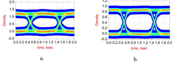
Fig. 10. Eye diagrams for a 6 mm long high density bus at 1 Gbps with the return path constrained (a.), with the return path a full plane (b).
