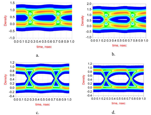
Fig. 9. Eye diagrams for a 6 mm long high density bus at 2 Gbps for different bus configurations.
