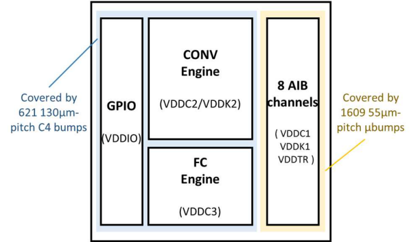
Fig 1. Chiplet functional block diagram.
