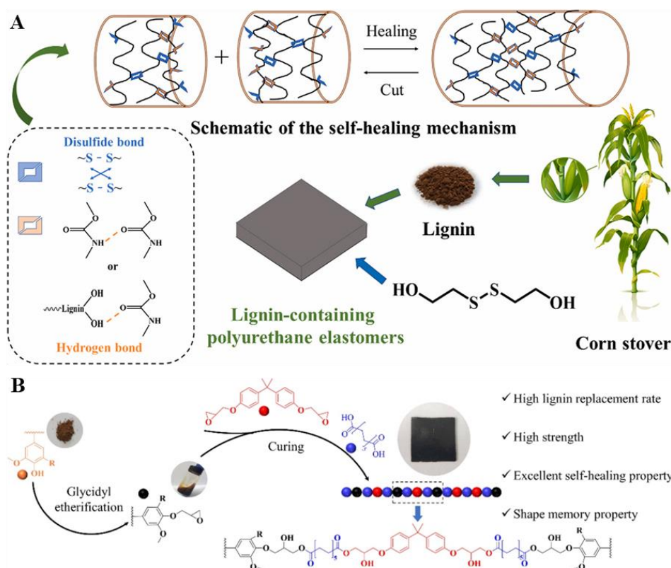
Figure 7. (A) Schematic overview of lignin-based PU with self-healing properties. 153 Copyright 2021, Elsevier. (B) Schematic overview of the development of lignin-based vitrimer as a sustainable alternative to bisphenol A epoxy resin. 155 Copyright 2021, Elsevier.
