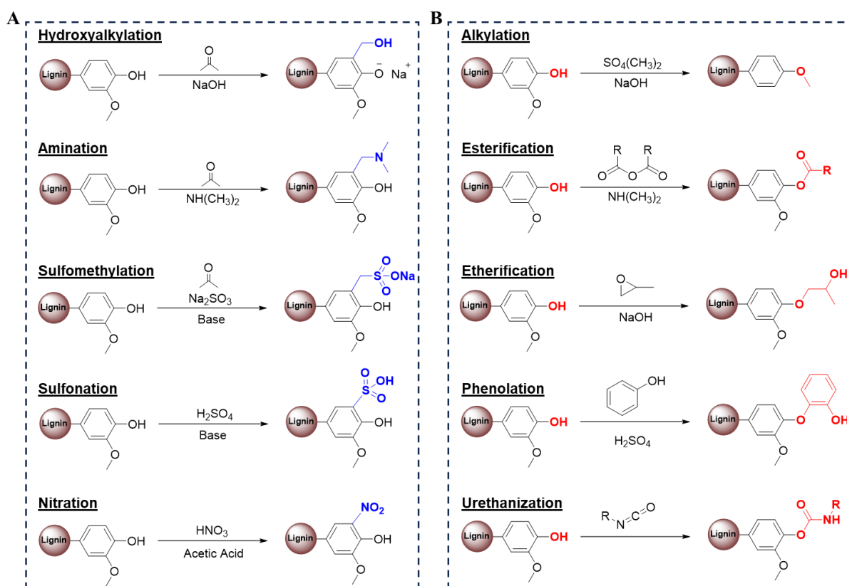
Figure 2. (A) Schematic overview of chemical modifications generating new active sites in lignin; (B) Schematic overview illustrating the functionalization of lignin's hydroxyl groups. 32 Copyright 2019, Elsevier.
