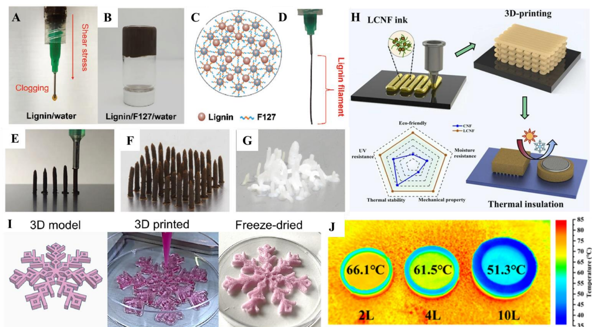
Figure 6. Direct ink writing (DIW) of lignin materials. A digital image of (A) the lignin/water ink and (B) the lignin/F127/water ink (with 50 wt% of lignin) stored in an inverted vial to demonstrate its high viscosity. (C) Schematic of the interaction of lignin with F127. (D) Digital image of a lignin/F127/water filament extruded from a syringe with improved lignin printability. (E, F) Images of the vertical printing of lignin and (G) cellulose (cellulose cannot form a free-standing structure via vertical printing). 66 Copyright 2020, Wiley-VCH. (H) Schematic illustration of the manufacturing
