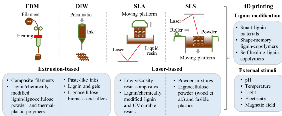
Figure 3. Scheme of different 3D printing techniques used for lignin-based materials and derived 4D printing of lignin materials. Materials extrusion: FDM and DIW; Laser-based: SLA and SLS.
