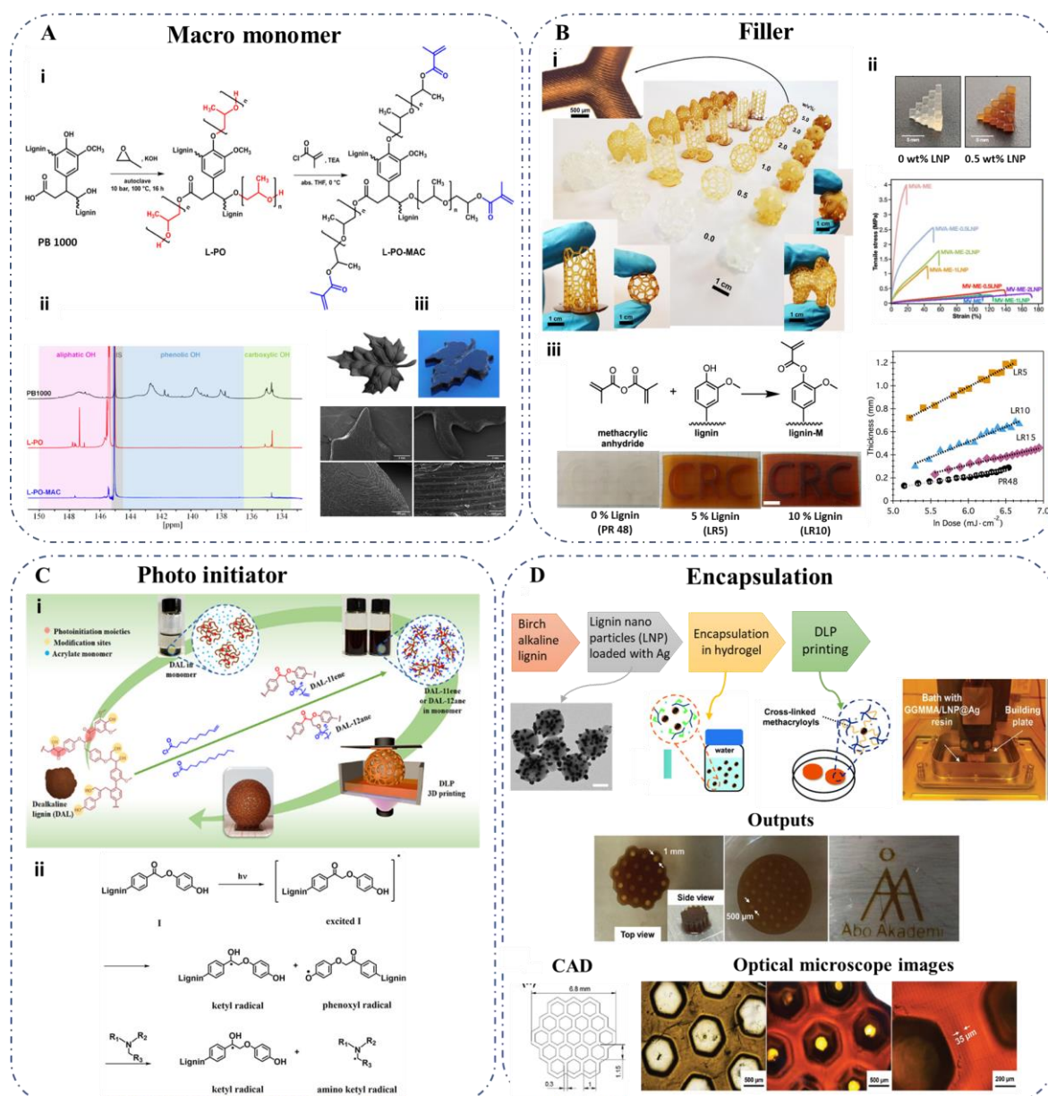
Figure 5. Utilization of lignin for SLA and DLP 3D printing categorized by the function of lignin. (A) Lignin as macromonomer: (i) Modification pathway of wheat straw lignin to generate photopolymerizable macromonomer (ii) ^{31}\text{P} -NMR spectra of Wheat straw soda lignin (PB1000), propoxylated lignin (L-PO), and methacrylated propoxylated lignin (L-PO-MAC) (iii) CAD render, printed maple leaf and SEM images of the show parts. 125 Copyright 2023, American Chemical Society. (B) Lignin as fillers: (i) Photos of 3D printed composites with kraft lignin copolymerized with PEGDA at 0-5 w/v% (Top left: Optical microscope image of sample 5 w/v%, 37 Copyright 2023, American Chemical Society. (ii) Photos of lignin nanoparticle (LNP) incorporated specimens and stress-strain curves indicating tunable strength and ductility profiles at different LNP loadings (0.5-2.0 wt%), polymer matrix (MV: Methacrylated vanillin, MVA: Methacrylated vanillyl alcohol, ME: Methacrylated eugenol), 64 Copyright 2023, Elsevier. (iii) Synthesis of methacrylated lignin and effect of methacrylated lignin addition in the layer thickness and print quality; scale bar is 1 cm. 20 Copyright 2018, American Chemical Society. (C) Lignin as photoinitiators: (i) grafting long alkane (DAL-12ane) and alkene (DAL-11ene) chains (ii) generation of free radicals in dealkaline lignin under light. 126 Copyright 2020, American Chemical Society. (D) Lignin for encapsulation: silver-lignin nanosphere
