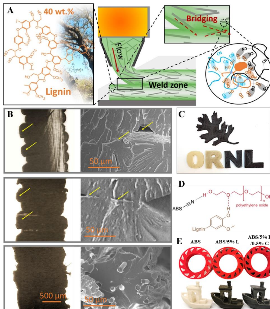
Figure 4. (A) Scheme to highlight the alignment of CF along the printing flow and CF bridging the weld zone. 89 Copyright 2018, Elsevier. (B) The cross-section optical images (left) and corresponding cross-section SEM images (right) of the 3D-printed samples: (top) ABS; (middle) ABS-NBR41-Lignin-514; and (bottom) ABS-NBR41-Lignin-CF-4141. The yellow arrows in the optical images (left) and in the SEM images (right), top and middle, indicate individual 3D-printed layers and un-fused areas, respectively. (For interpretation of the references to color in this figure legend, the reader is referred to the web version of this article.). 89 Copyright 2018, Elsevier. (C) Examples of 3D-printed objects made from ABS (“O” and “R”), ABS-NBR41-Lignin-514 (“N”), and ABS-NBR41-Lignin-CF-4141 (“L” and the oak leaf). 89 Copyright 2018, Elsevier. (D) The hydrogen-bonded network of lignin with PEO in the ABS matrix. 90 Copyright 2015, American Chemical Society. (E) The filament rolls at different composition ratios of ABS, lignin (L), and graphene (G); the quality of 3D printed objects. 91 Copyright 2021, Wiley-VCH.
