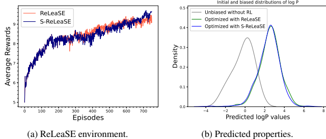
Fig. 4: Performance of the generator fine-tuned with RL. Example of two generated molecules: SMILES - BrC1cccc1, C=C(C=CC)Sc1cccc1 with logP values 2.45 and 3.87, respectively.
