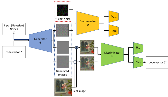
Fig. 5. Adjustment to the training for denoising experiment.
