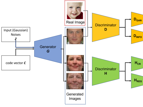
Fig. 1. Proposed Architecture. Building upon InfoGAN-CR [8], we add additional regression layer that quantify the similarity (or differences) of the input images attributes
