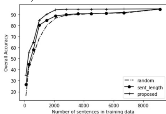
Figure 3. Comparison of different annotation methods
