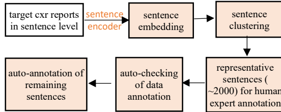
Figure 1. Proposed weak supervision annotation framework. Sentence Encoder is on our CXR data. Auto-checking checks the inconsistency and bias in the human annotation.
