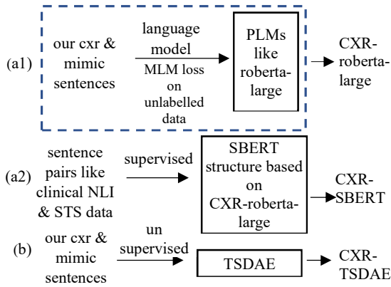
Figure 2. Supervised Sentence Encoder Training : (a1) to get domain adapted model (CXR-Roberta-large) through behavior fine tuning on pretrained model; (a2) further trains the adapted model (CXR-Roberta-large) to obtain a supervised sentence encoder (CXR-SBERT) on labelled clinical NLI or STS data.
