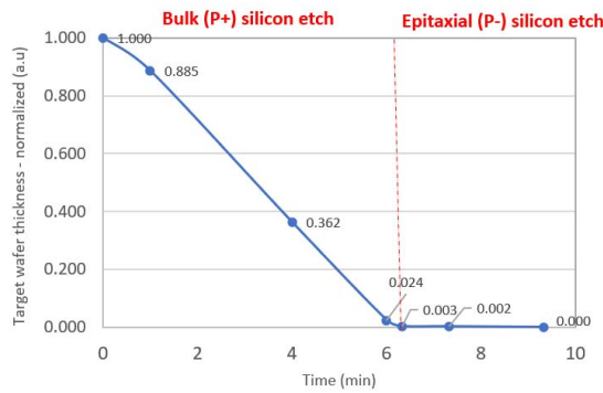
Fig. 3: Evolution of target wafer thickness (normalized and expressed in arbitrary units) etched in composition 2, showing linear etch in bulk silicon and etch stop at the epitaxial film interface.
