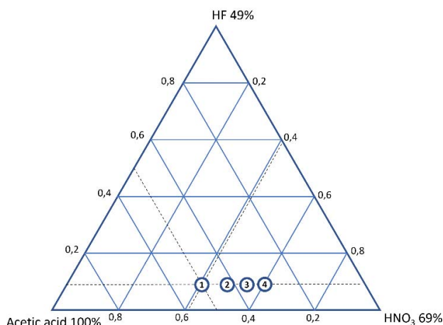
Fig. 2: HNA mixing triangle representing various compositions studied in this work.
