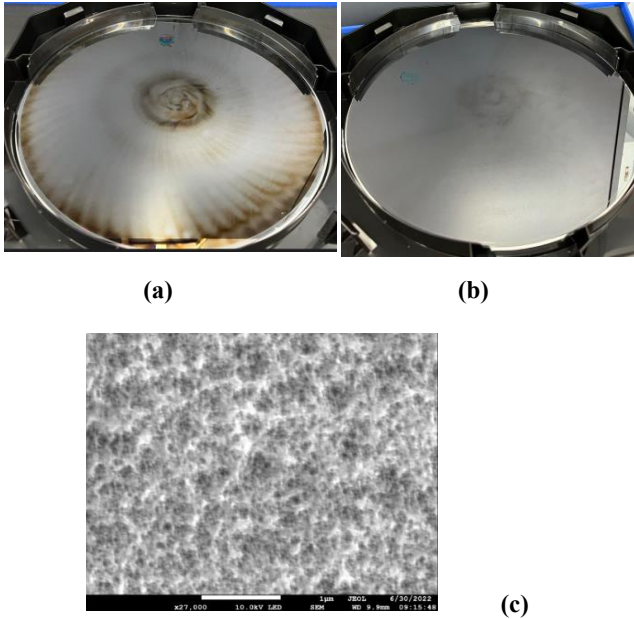
Fig. 5: Optical images showing (a) brown staining on the etched wafer surface during the process, (b) brown staining mitigated with overetching on the same wafer, (c) SEM image of the wafer staining
