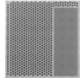
Fig. 12: Xray image on good solder alignment after TCB bonding process
