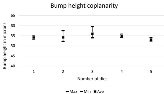
(c) Daisy chain test chips for 3 die chiplet Fig. 4: Bump height coplanarity
