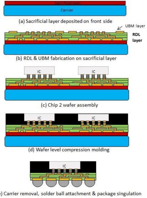
Fig. 2: Overall Assembly Process Flow
