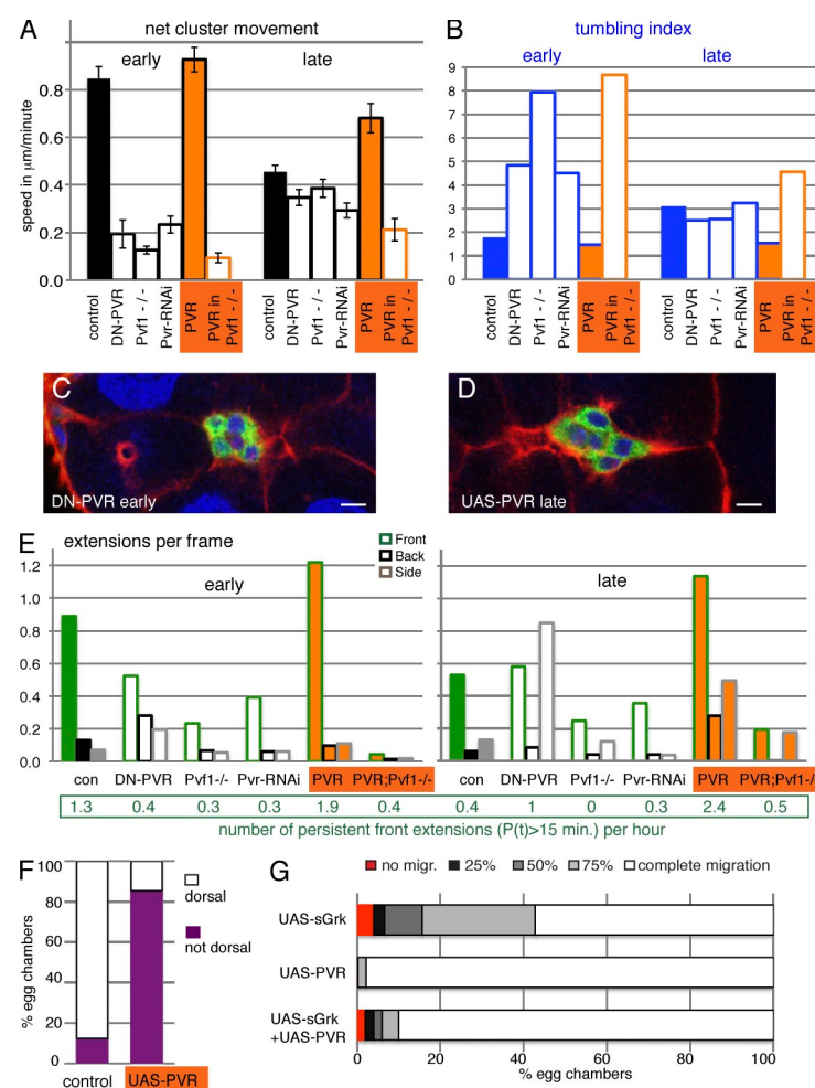
Figure 4. Effects of PVR on the behavior of border cell clusters.
