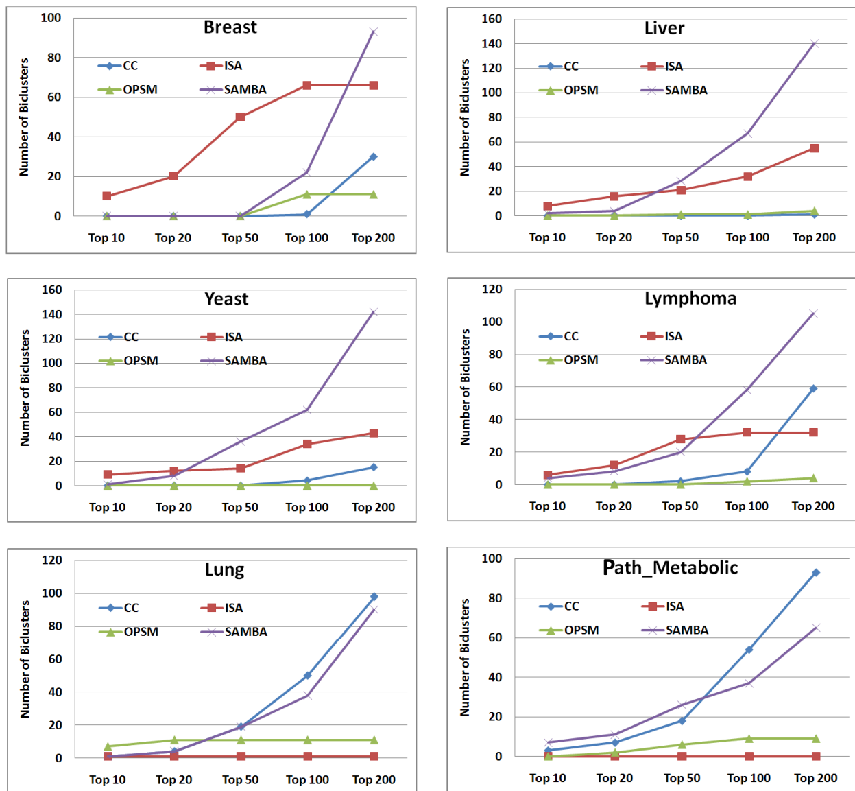
Figure 6 Rank distribution of biclusters. Rank distribution of the biclusters from each algorithm in a combined ranking on different datasets.
