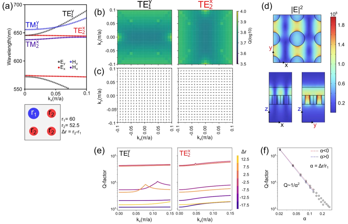
Figure 2. Mode analysis for BZF structure with a finite radius perturbation. (a) Calculated band structure for both TE and TM modes of a 2x2 supercell with (r_1, \Delta r) = (60, -7.5) nm along \Gamma \rightarrow X' . (b) 2D k -space maps of Q-factor and (c) far field polarization maps of near \Gamma point of TE_1^y (left) and TE_2^x (right) for (r_1, \Delta r) = (60, -7.5) nm. (d) Corresponding mode profile |E|^2 of TE_1^y mode at \Gamma point along xy (middle height of TiO_2 cylinders), xz and yz planes. (e) Simulated Q factor of TE_1^y and TE_2^x modes with r_1 = 60 nm and \Delta r varying from -17.5 nm to 12.5 nm along k_x . (f) Q-factor at \Gamma point scales with the asymmetry factor ( \alpha = \Delta r/r_1 ) showing the Q \propto 1/\alpha^2 dependence. The Q-factor dependence differs slightly with the sign of \alpha , likely due to the simplified definition of \alpha .
