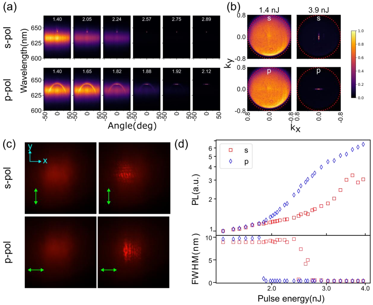
Figure 3. Lasing characteristics of the BZF-GR mode for the lowest threshold array ( r_1, \Delta r ) = (60, -2.5) nm. (a) Power dependent normalized PL spectra for s- and p-polarized emissions. Numbers in each graph indicate the incident pumping pulse energy on the sample in nJ. (b) Back focal plane images for s- and p-polarized emissions at low (1.4 nJ) and high (3.9 nJ) pumping pulse energies. (c) Optical images of the array at low (left) and high (right) pumping pulse energies under different polarizer alignments. The polarizer alignment, along with the polarization labelling is in the bottom left of each image. (d) Integrated PL emission (top) and FWHM (bottom) plotted against pumping pulse energy.
