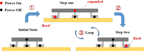
Fig. 5. Robot locomotion.
