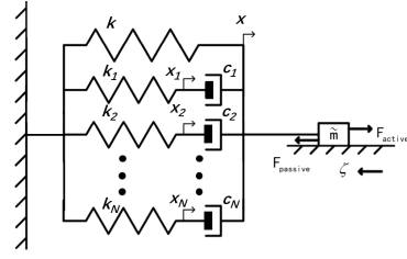
Fig. 6. Dynamic model of the DEA
