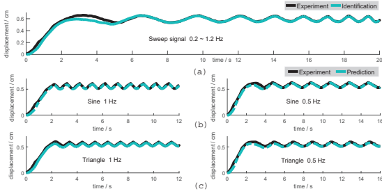
Fig. 7. Experimental results of model identification with validation. (a) identification result applying a sweep voltage signal, (b) (c) validation results applying sine voltage signals and triangle voltage signals, respectively.
