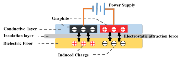
Fig. 4. Working principle of the EA.
