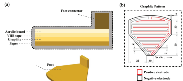
Fig. 3. Schematic of the robot foot. (a) exploded view, (b) dimensions of the electrode pattern.
