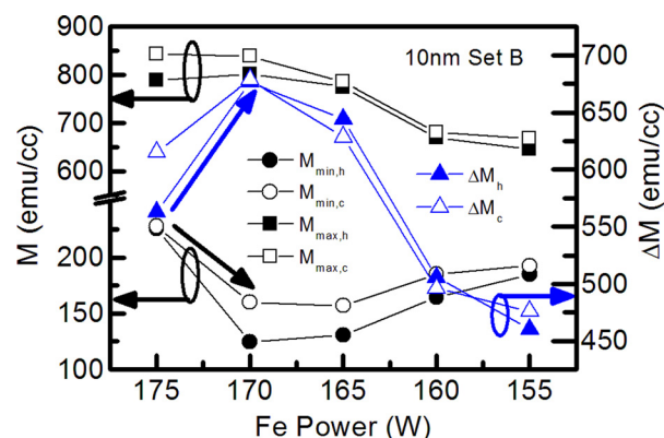
FIG. 8. Transition parameters M_{min} , M_{max} , and \Delta M extracted from Figure 7 (10 nm sample Set B).
