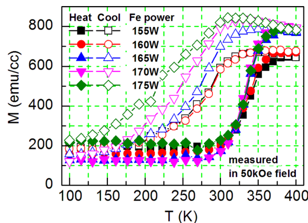
FIG. 7. M-T plots for 10 nm sample Set B.
