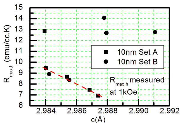
FIG. 12. R_{\text{max,h}} of samples showing linear dependence with c and 4 outlier points that departs from this linearity when grain sizes were large, crystallinity were improved, and Fe content were high.
