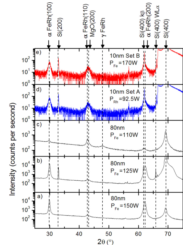
FIG. 1. Typical XRD profiles of 80 nm sample set (a)–(c), 10 nm sample Set A (d), 10 nm sample Set B (e).
