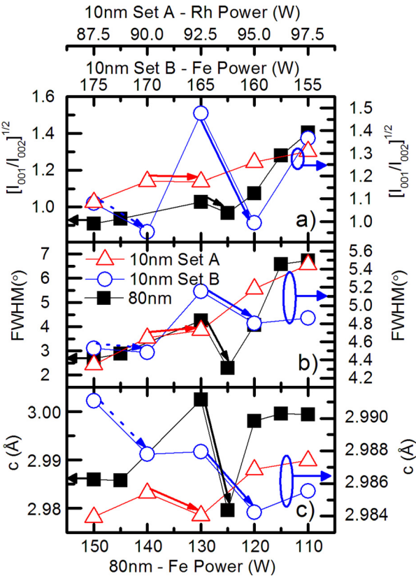
FIG. 3. Parameters extracted from XRD profiles for the 80 nm sample set and 10 nm sample sets.
