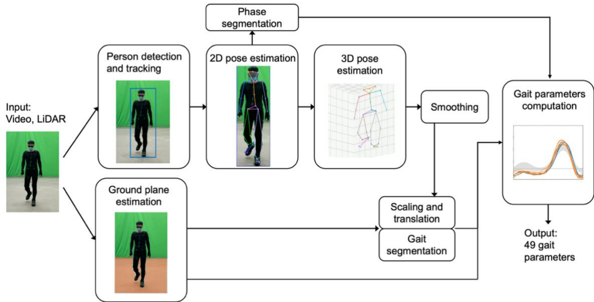
Fig. 1. Architecture of 3DGait.
