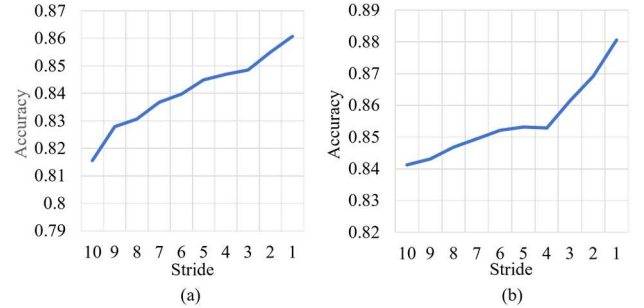
Fig. 3. The impact of convolved stride to prediction accuracy. (a) and (b) shows the result form IMU HAR dataset [5] and [10] accordingly.
