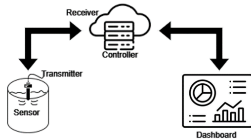
Figure 1 Cyber-physical water monitoring system
