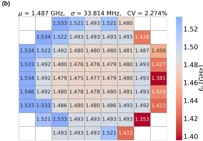
Fig. 2. (a) One port S_{11} measurement showing the magnitude (dB) and phase (deg) variation with frequency of the BAW array. Inset shows the zoom-in around the resonance with cavity mode separation of 5.6 MHz. (b) Wafer-level heat-map showing the variation in resonance frequency with position. The mean value of resonance, standard deviation and coefficient of variation are 1.487 GHz, 33.8 MHz, and 2.27% respectively.
