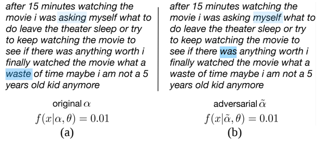
Fig.4. Heatmap illustrating the attention weights generated from a negative movie review [37] . (a) Attention weights. (b) Adversarially constructed set of attention weights.
