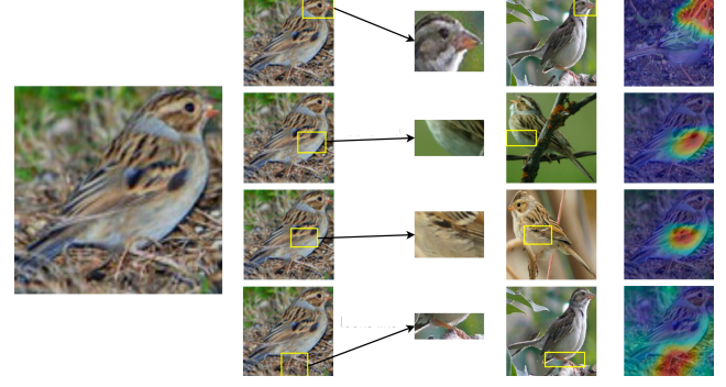
Fig.5. This figure demonstrates a prototype-based explanation. It features a test image of a clay-colored sparrow in the first column. The third column highlights the similar regions between the test image in the first column and the prototype depicted in the fourth column, while the rightmost column presents the corresponding activation map, illustrating the basis for the model's prediction.
