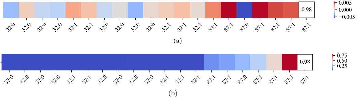
Fig.8. Visualization of explanation in knowledge tracing on ASSISTment 2009. (a) KernelSHAP. (b) Attention.
