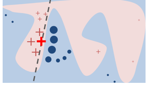
Fig.3. LIME example [34] . The pink/blue background signifies the presence of the black-box model, while the prominent red cross serves to identify the instance undergoing explanation. The remaining red crosses and dots represent data points acquired through sampling, with their sizes reflecting their similarity to the specific instance being explained.
