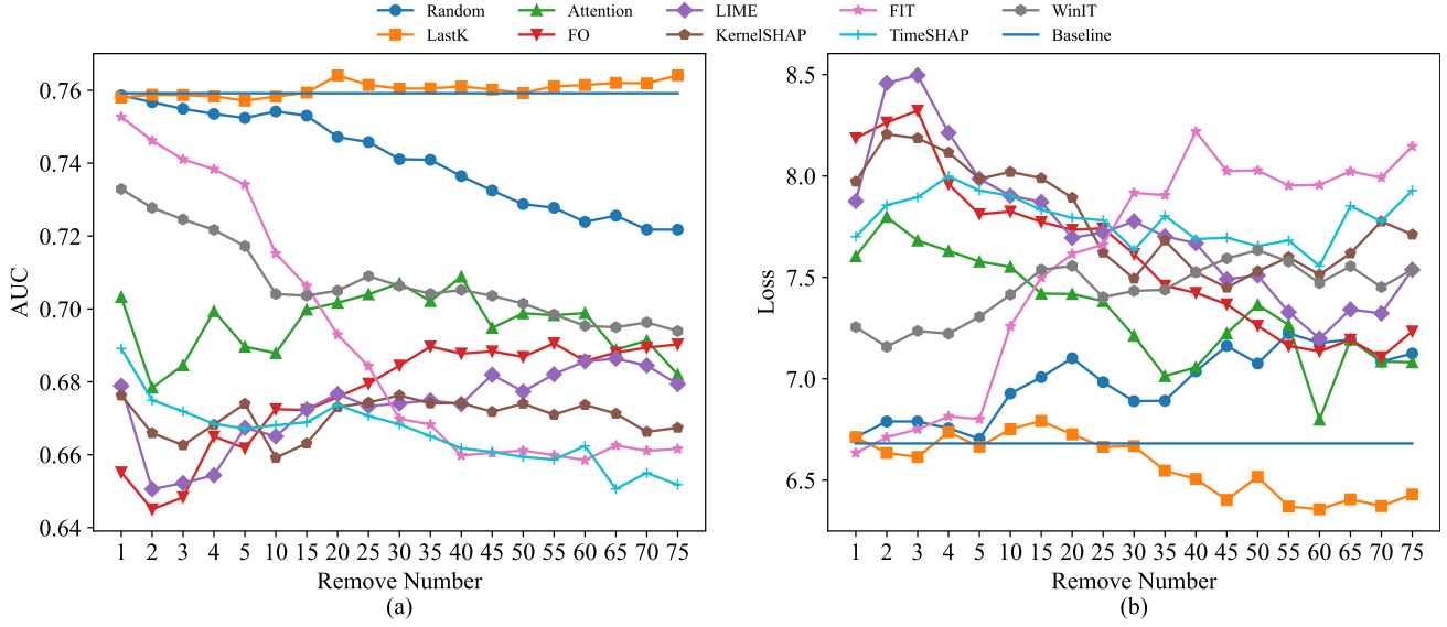
Fig.7. The performance of explanation methods varies with the increase in K on ASSISTment 2017, where the Baseline refers to the model performance with no features removed. (a) AUC. (b) Loss.
