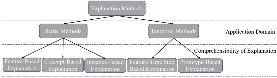
Fig.1. Overview of our taxonomy.
