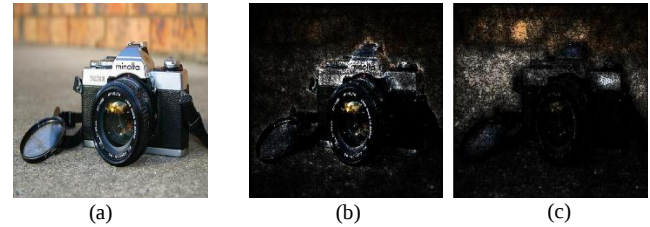
Fig.2. Example of saliency map generated by Integrated Gradients and Gradient. (a) Original image. (b) Integrated Gradients. (c) Gradients.
