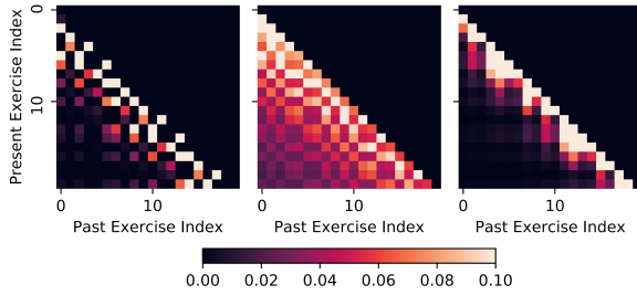
Fig.6. The attention weights of the three attention heads in AKT.
