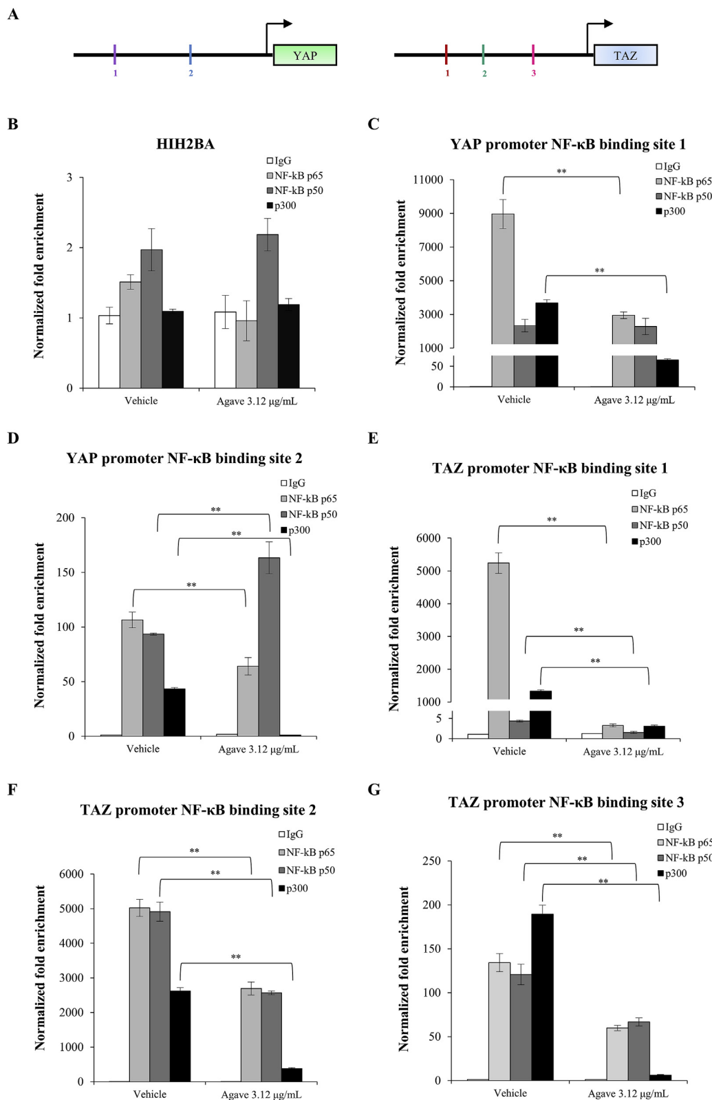
Fig. 6. Agave inhibits NF- \kappa B recruitment onto YAP and TAZ promoters. (A) Schematic representation of the relative position of the putative NF- \kappa B binding sites within the YAP and TAZ promoters. Different sites are highlighted in different colors, which are consistent with that used for sequences showed in Supplementary Figs. S2I–J . U-2 OS cells were treated with Vehicle (EtOH) or Agave (3.12 \mu g/mL) for 72 h before being analyzed by ChIP. Samples were immunoprecipitated with antibodies against IgG, NF- \kappa B p65, NF- \kappa B p50 or p300 and then subjected to qPCR analysis. Histograms shows the mean fold enrichment \pm STDEV ( n = 3 ) for HIH2BA (B) , and the putative NF- \kappa B binding sites within the YAP (C–D) and TAZ (E–G) promoters, ANOVA **p < 0.001 . (For interpretation of the references to color in this figure legend, the reader is referred to the Web version of this article.)
