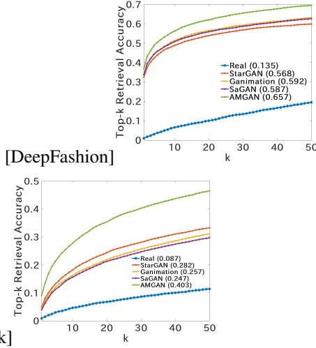
Figure 4. Average Top-K retrieval accuracy of attribute manipulations. The number in the parentheses corresponds to the Top-30 retrieval accuracy.
