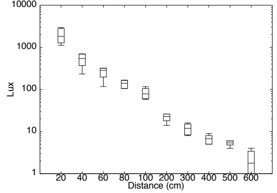
Fig. 12. Light Intensity vs. distance using a 9 W LED and light sensor on Galaxy S II.
