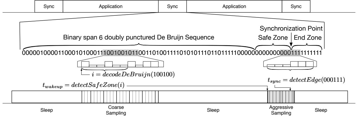
Fig. 5. A doubly punctured De Bruijn sequence emitted as preamble. All the duty-cycling devices sample the ambiance and get synchronized on the peak while transiting from the safe zone to the end zone.
