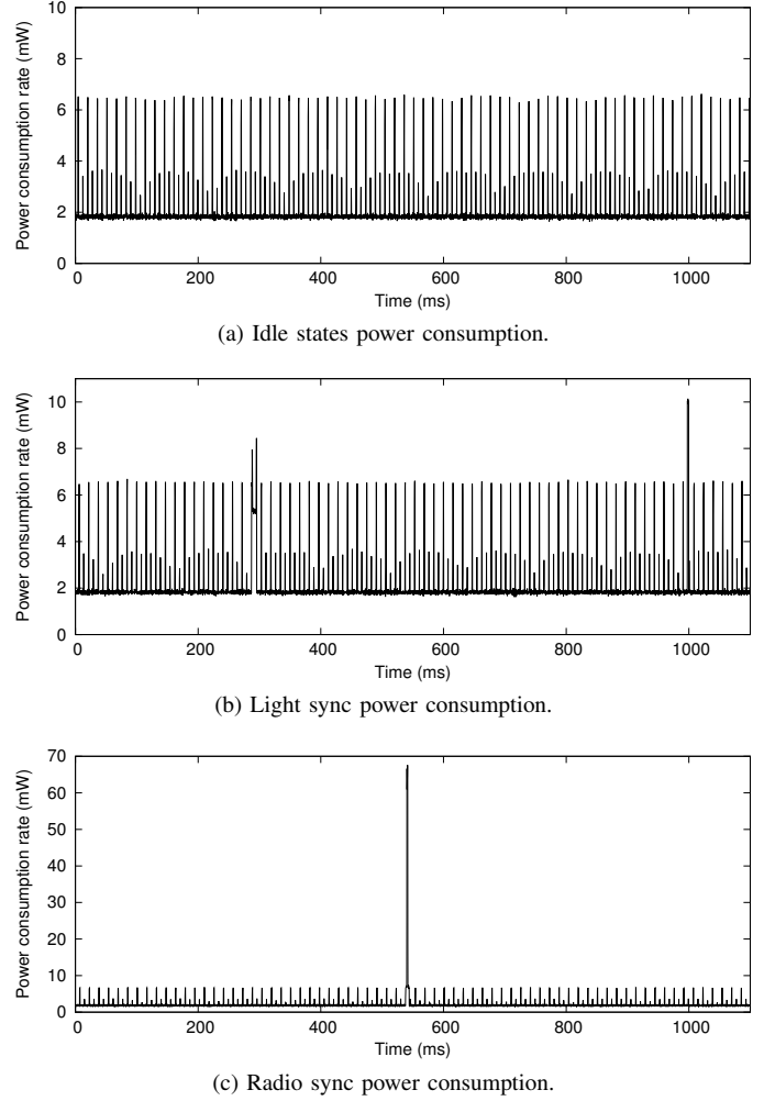
Fig. 10. Power profiles for different operations: (a) CPU idle, (b) running PSync every second, (c) reception of a 1-byte packet over IEEE 802.15.4 radio.
