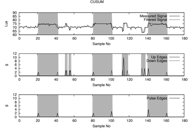
Fig. 7. Edge detection algorithm.
