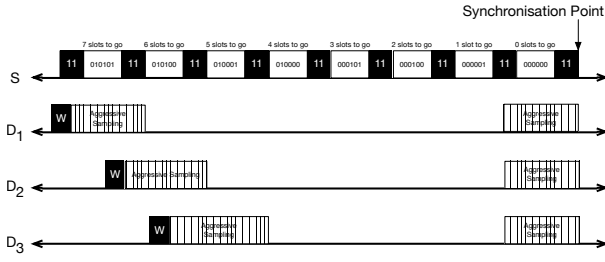
Fig. 4. A slotted preamble with encoded data allowing higher duty cycling.
