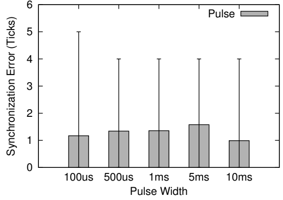
Fig. 9. Impact of pulse width, when synced with pulse.
