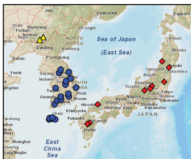
Fig. 1 Geographical distribution and principal component (PC) analysis of population genetic structure for 138 Miscanthus sinensis genotypes using 14 073 single-nucleotide variant loci. The percentages of the total variation explained by each PC are shown in parentheses.
