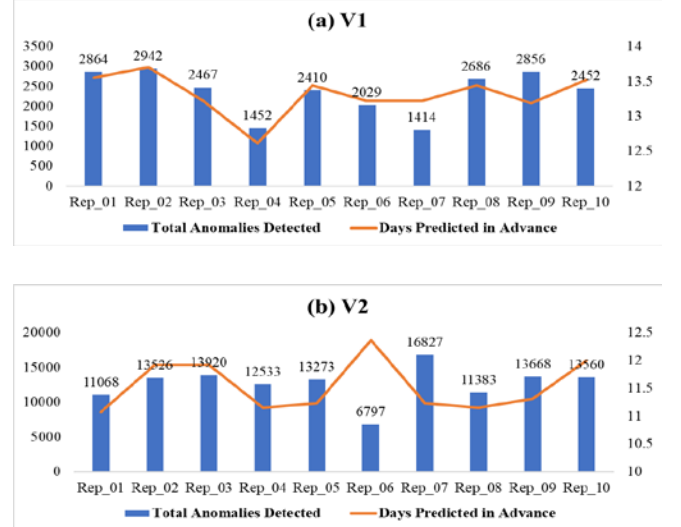
Fig. 7. Total Anomalies Detected and Days Predicted in Advance
