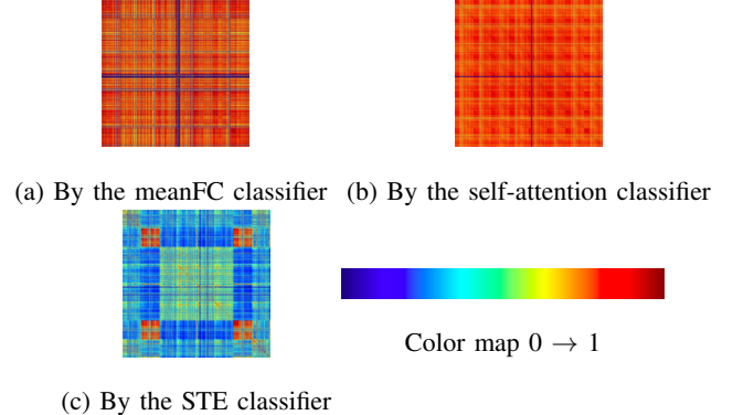
Fig. 1: The heat maps of Pearson correlation coefficient score among encoded features extracted by the pre-trained model VideoViT [1] when it combines with (a) meanFC, (b) self-attention, and (c) our proposed head (STE) as a classifier.
