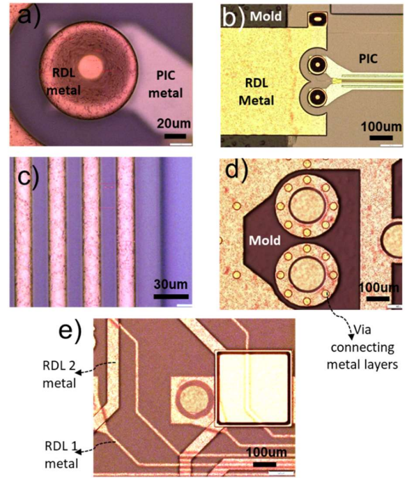
Fig. 9. Images of package RDL processing a) via connecting PIC metal to package RDL metal. b) Metal connecting PIC to the fanout area. c) Package metal interconnects with line/space of 15um/15um d) high-speed metal interconnects from modulators on mold area. e) image showing RDL 1 and RDL 2 metal.
