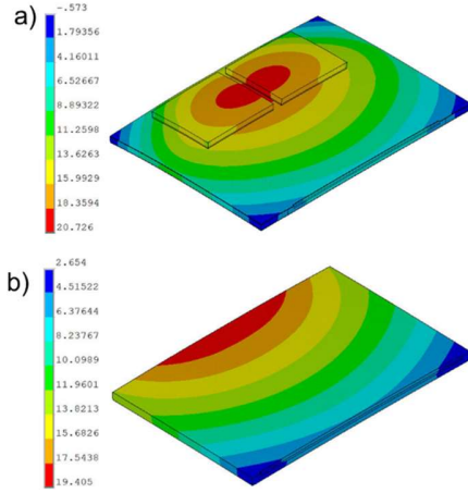
Fig. 4. a) Warpage ( \mu m) of optical engine package. b) Warpage ( \mu m) of PIC die embedded in the mold.
