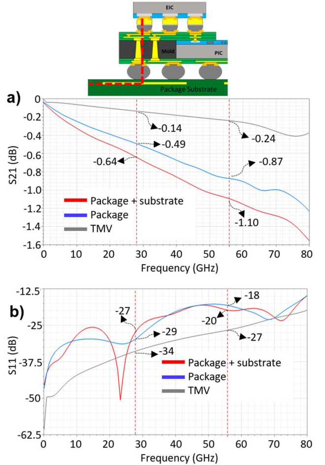
Fig. 3. a) Plot showing the frequency response of the differential transmission interconnects connecting the substrate to the input of the EIC (driver) including the \mu\text{bump} , front side RDL, TMV, backside RDL, c4 bump and substrate a) insertion loss b) reflection loss.
