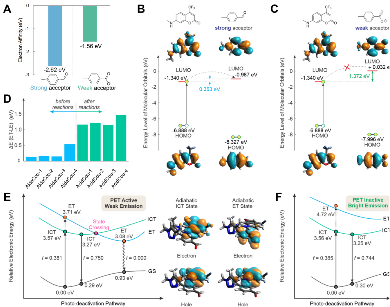
Figure. 4 Theoretical calculations to rationalize the fluorescence turn-on mechanism. (A) Calculated electron affinity of the benzaldehyde and benzoate moieties in water. Comparison of the energy levels of frontier molecular orbitals between coumarin and (B) benzaldehyde, or (C) benzoate in water. (D) Calculated energy gaps between the high-lying electron transfer (ET) and low-lying intramolecular charge transfer (ICT) states in the four probes and their corresponding oxidized products during vertical excitations. (E) Schematic illustration of the state-crossing from an ICT to an ET state and calculated excitation/de-excitation energy (as well as oscillator strength, f ) of AldeCou-1 in water; the inset shows the corresponding electron and hole distributions of the adiabatic ICT and ET states. (F) Schematic illustration of the potential energy surface and calculated excitation/de-excitation energy (as well as oscillator strength, f ) of AcidCou-1 in water. The energy levels are not drawn to scale in (E) and (F) for improved clarity.
