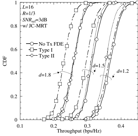
Fig. 3. Impact of Tx FDE weights at S during broadcast phase.
