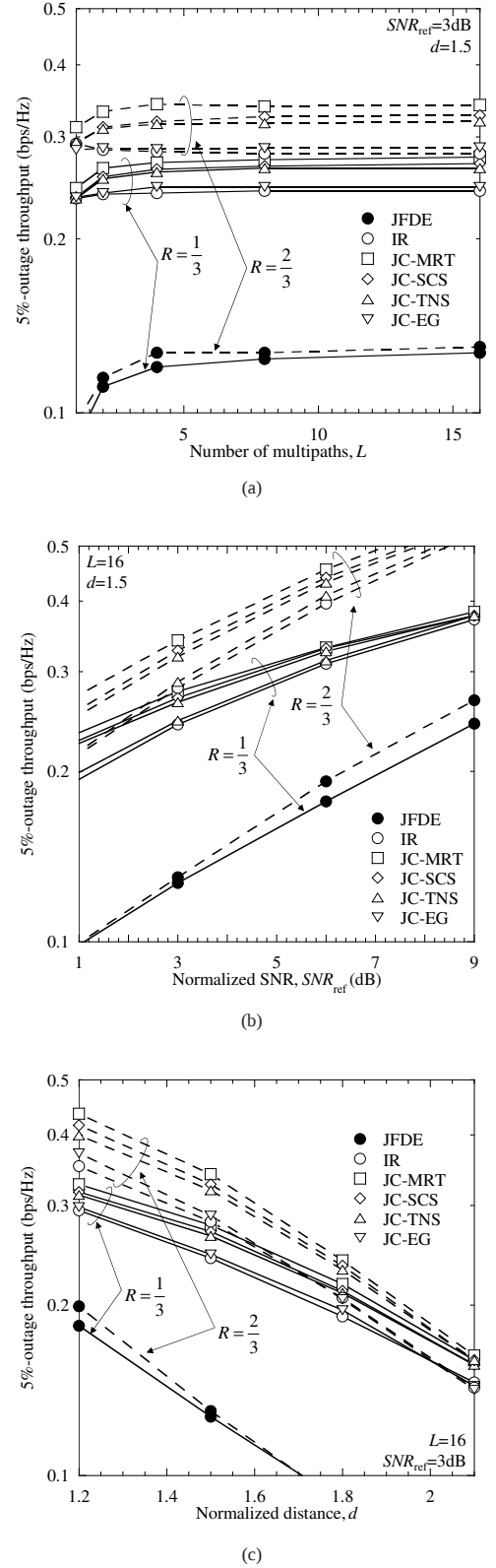
Fig. 5. Impact of channel model (a) Number of multipaths, L (b) Normalized SNR, SNR_{\text{ref}} (dB) (c) Normalized distance, d .
