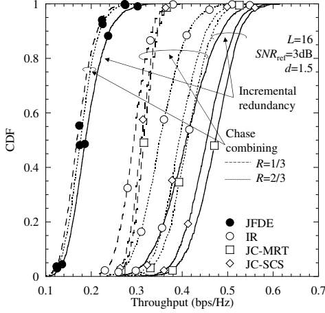
Fig. 6. Throughput performance with different HARQ strategies.
