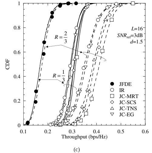
Fig. 4. Performance improvement obtained by the proposed joint cooperative-Tx/Rx FDE (a) Required number of retransmissions per packet for correct decoding (b) Packet loss rate (c) Throughput (bps/Hz) .
