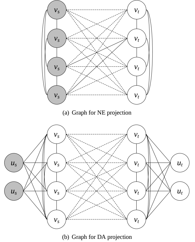
Fig. 3. Graph Structures for Cross-lingual SLU
