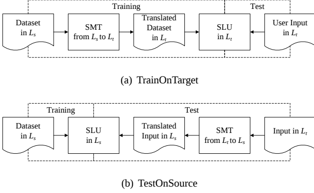
Fig. 1. Cross-lingual SLU strategies
