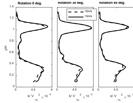
Fig. 6. Normalized turbulence kinetic energy at 2H downstream.
