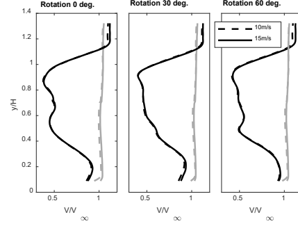
Fig. 4. Normalized wake profile at 1H upstream (grey) and 2H downstream (black)
