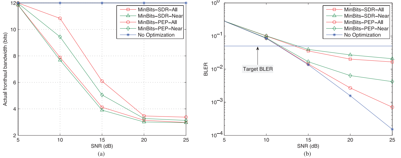
Fig. 7. Performance comparison between all-symbol scheme and nearest-symbol scheme. 4-PAM modulation, N = M = 2 . Average fronthaul bandwidth is equal to 12 bits. (a) Compression efficiency. (b) BLER performance.
