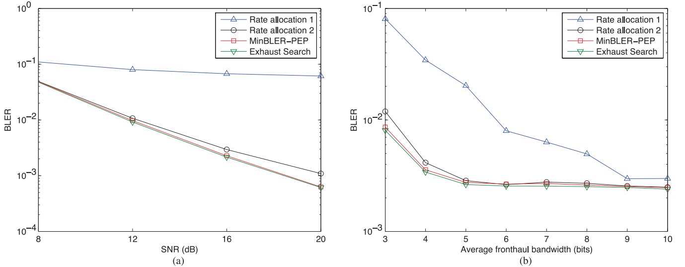
Fig. 6. BLER comparison of the optimal rate allocation scheme for different Q_{sum} . Rate allocation 1: [Q_1, Q_2, Q_3] = [n, n, n] , Rate allocation 2: [Q_1, Q_2, Q_3] = [n-2, n, n+2] , where n is the average fronthaul bandwidth. In Fig. a, Q_{sum} = 9 . In Fig. b, SNR = 12 dB. (a) BLER v.s. SNR. (b) BLER v.s. fronthaul bandwidth.
