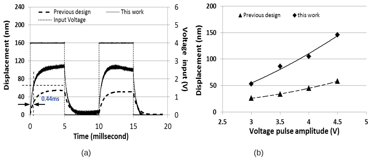
Fig.6 Step response under a 4V square voltage pulse input with 5ms pulse width at 50% duty cycle: (a) transient displacement and square voltage pulse over time; (b) steady-state displacement amplitude as a function of voltage pulse amplitude for the present and previous designs
