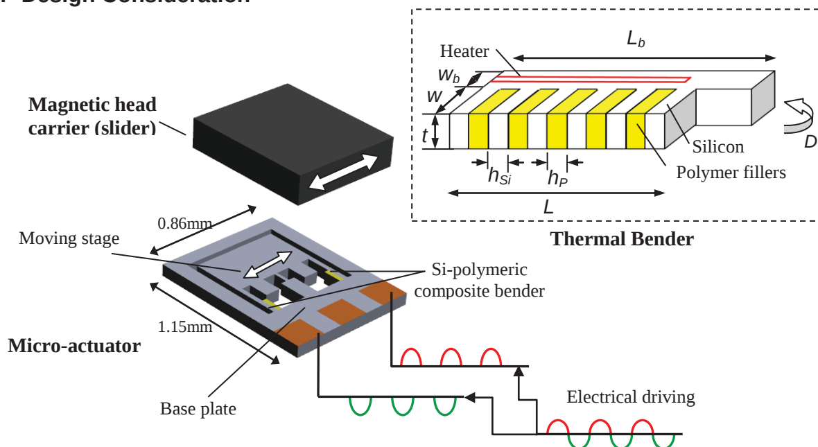
Fig. 1 Schematic of a micro-actuator carrying a magnetic head slider: each of the composite benders is electrothermally activated by a supply of half-sine voltage pulses
