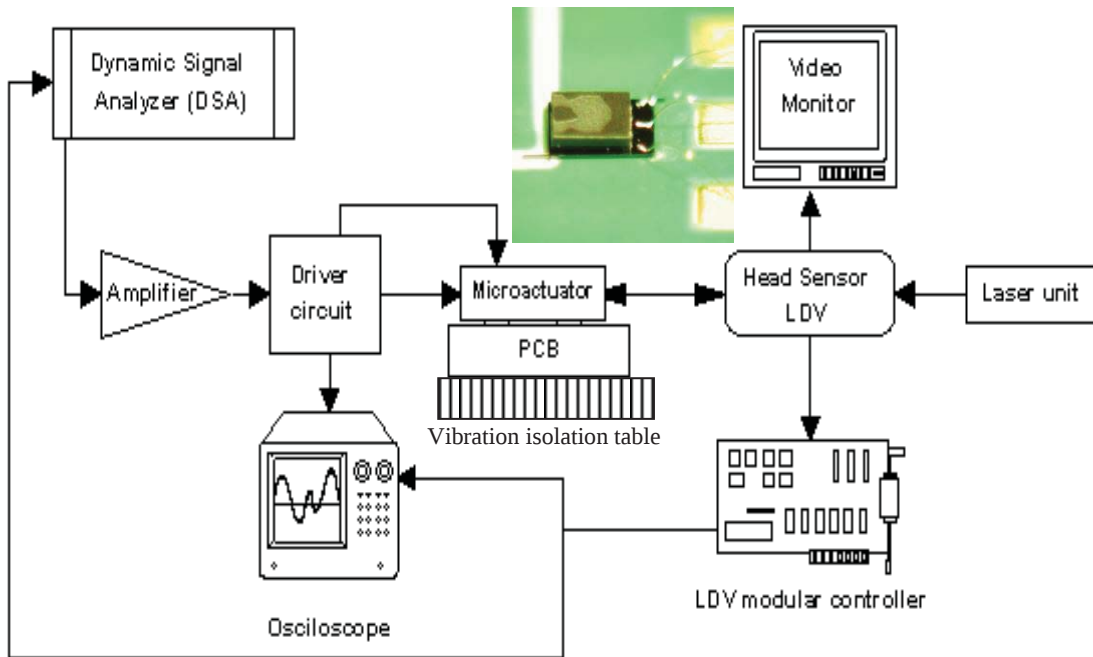
Fig. 5 Experimental setup of the device prototype on the PCB and vibration isolation table with a LDV system and electrical driving circuits
