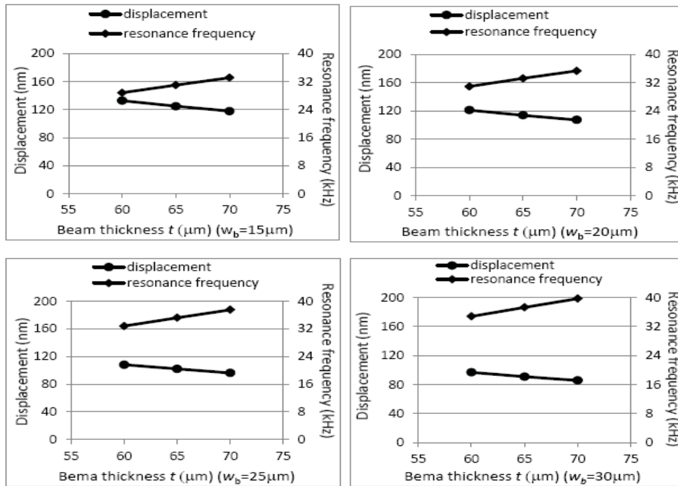
Fig. 3 Simulated displacements and frequencies varying with the beam thickness
