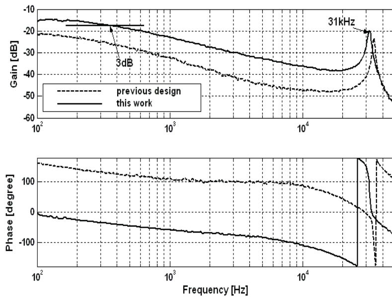
Fig. 8 Frequency response of the micro-actuator with a femto slider attachment
