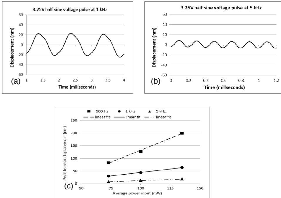
Fig. 7 Bi-directional time response of the slider under the excitation by 3.25V half sine voltage pulse at different driving frequencies: (a) time response under excitation at 1 kHz, (b) time response under excitation at 5 kHz and (c) the peak-to-peak dynamic displacement as a function of average input power at various excitation frequencies
