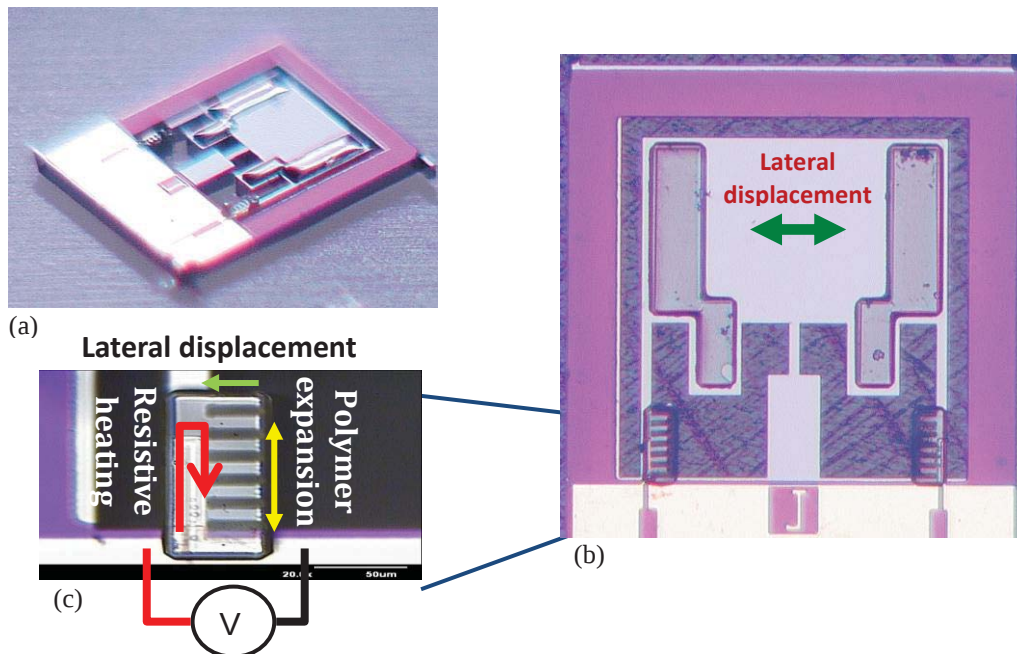
Fig. 4 Micrographs of the electrothermal micro-actuator with enhanced displacement: (a) optical micrograph of the 3D view of the micro-actuator, which consists of a moving stage, two composite benders and a central pivotal beam; (b) optical micrograph of top view of the micro-actuator; (c) close-up optical micrograph of the left composite bender which shows transparent SU-8, silicon comb and a resistance heater.
