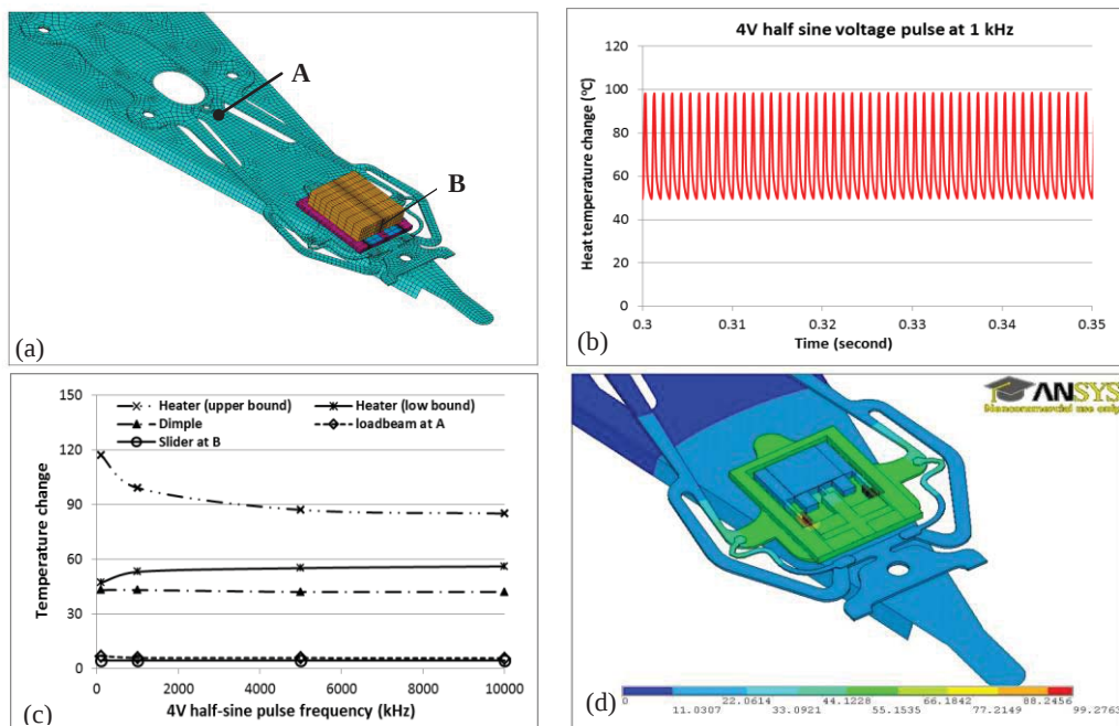
Fig. 9 Thermal simulation: (a) finite element model; (b) heat temperature responses by 4V half sine voltage pulse at 1 kHz; (c) transient temperature responses as a function of driving voltage frequency; (d) temperature distributions by 4V half sine voltage pulse at 1 kHz
