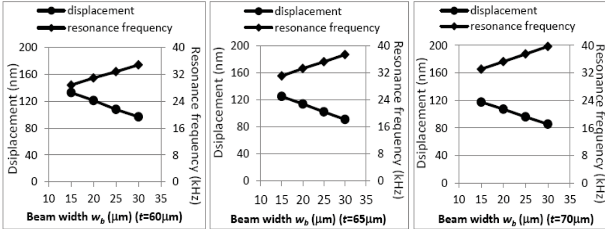
Fig. 2 Simulated displacements and frequencies varying with the beam width
